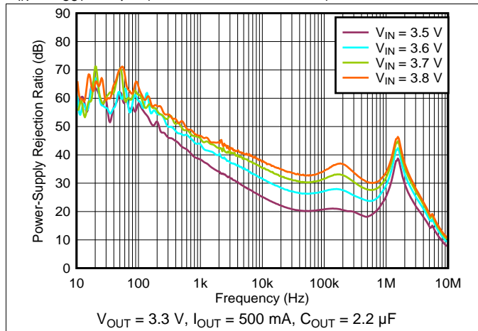
图 25. PSRR vs Frequency and V_{IN}
