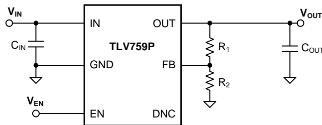
图 40. Adjustable Operation
