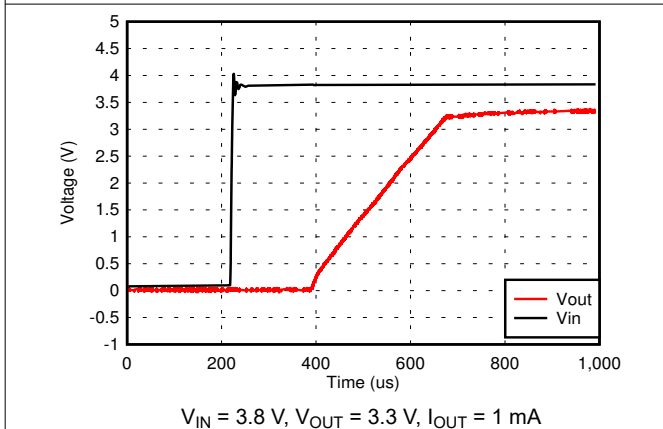
图 5-23. V_{IN} Power-Up
