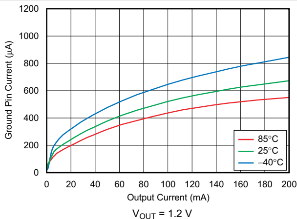
图 6-23. Ground Pin Current vs Output Current
