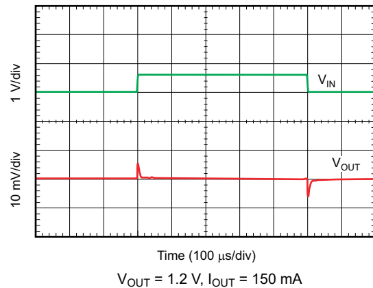
图 6-46. Line Transient Response
