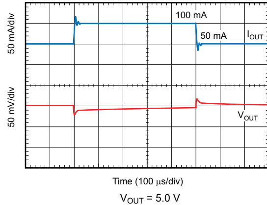
图 6-44. Load Transient Response
