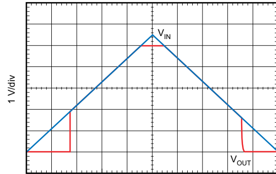
图 6-56. V_{IN} Ramp Up, Ramp Down Response
