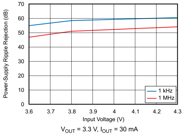
图 6-37. Power-Supply Ripple Rejection vs Input Voltage
