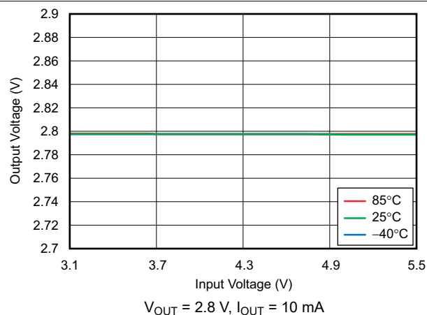
图 6-5. Line Regulation
