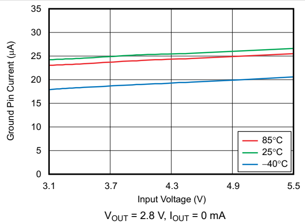
图 6-18. Ground Pin Current vs Input Voltage
