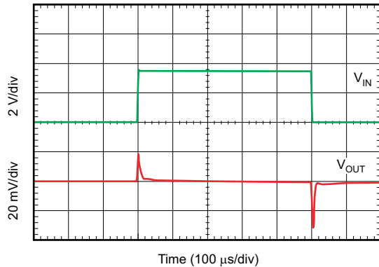
图 8-8. Line Transient Response
