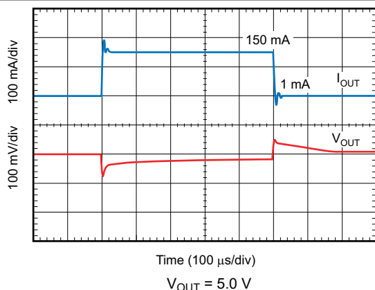
图 6-45. Load Transient Response
