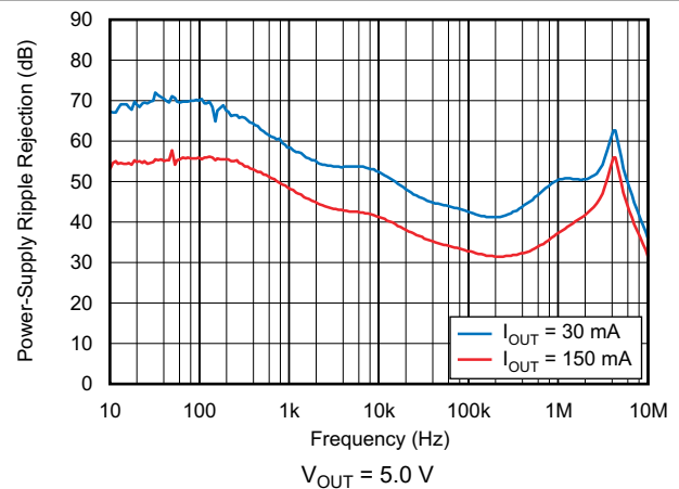
图 6-34. Power-Supply Ripple Rejection vs Frequency
