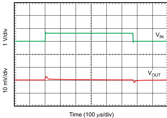
图 6-49. Line Transient Response
