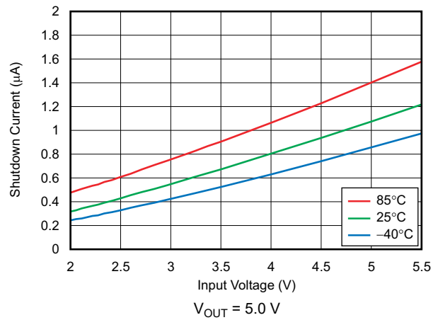
图 6-28. Shutdown Current vs Input Voltage
