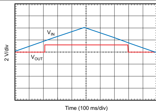
图 6-52. Line Transient Response
