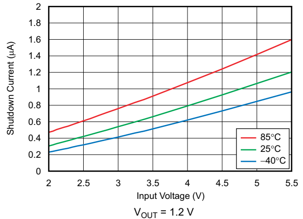
图 6-26. Shutdown Current vs Input Voltage
