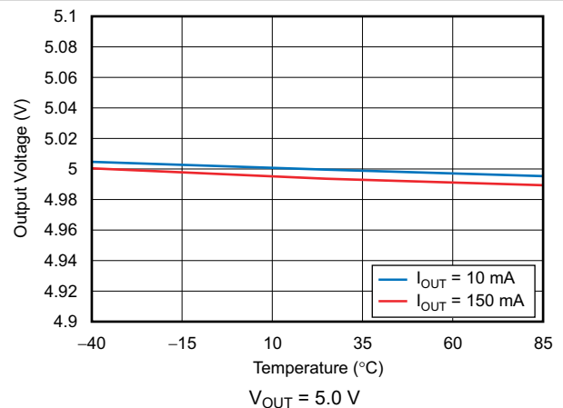
图 6-12. Output Voltage vs Temperature
