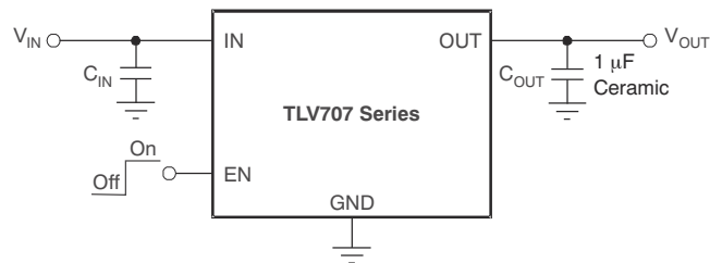
图 8-1. Typical Application Circuit
