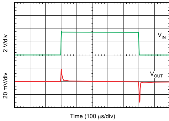
图 6-49. Line Transient Response
