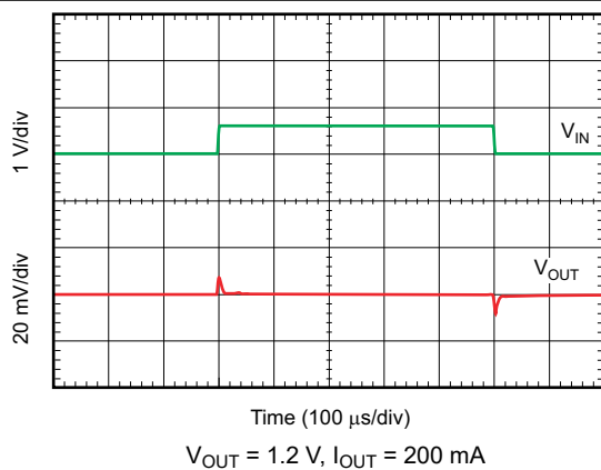
图 8-6. Line Transient Response
