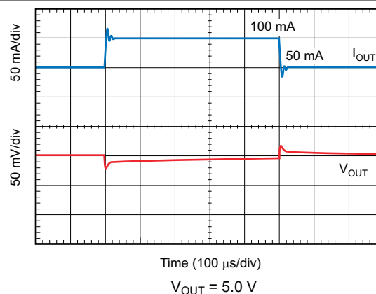
图 6-44. Load Transient Response
