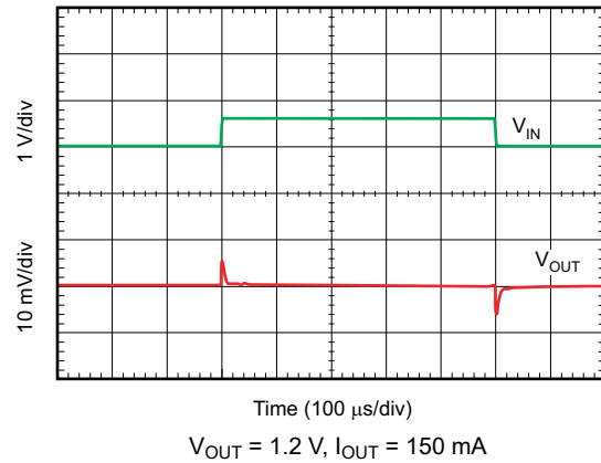
图 8-5. Line Transient Response
