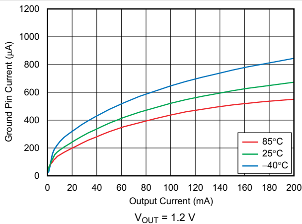
图 6-23. Ground Pin Current vs Output Current
