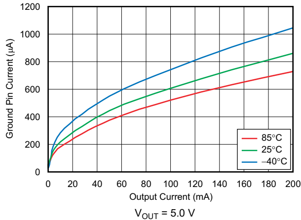
图 6-25. Ground Pin Current vs Output Current
