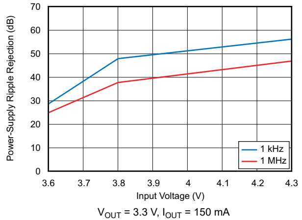
图 6-38. Power-Supply Ripple Rejection vs Input Voltage
