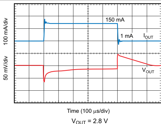
图 6-43. Load Transient Response
