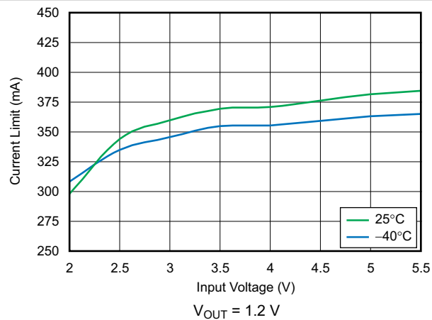
图 6-29. Current Limit vs Input Voltage
