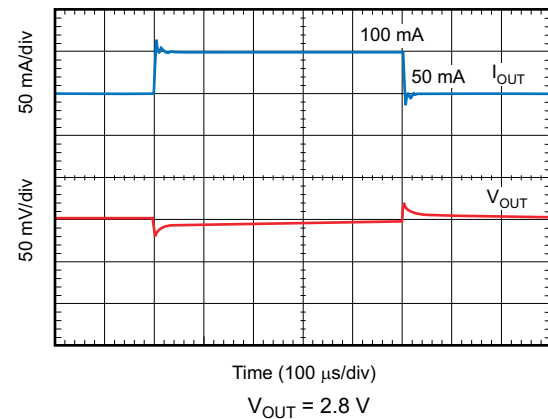
图 6-42. Load Transient Response
