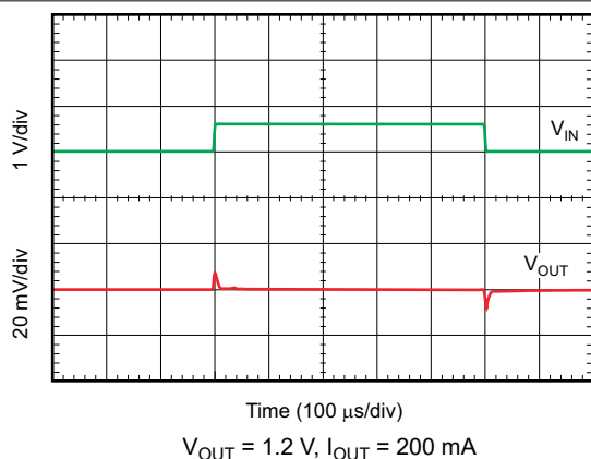
图 6-47. Line Transient Response
