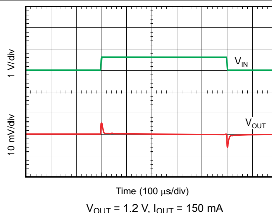
图 6-46. Line Transient Response
