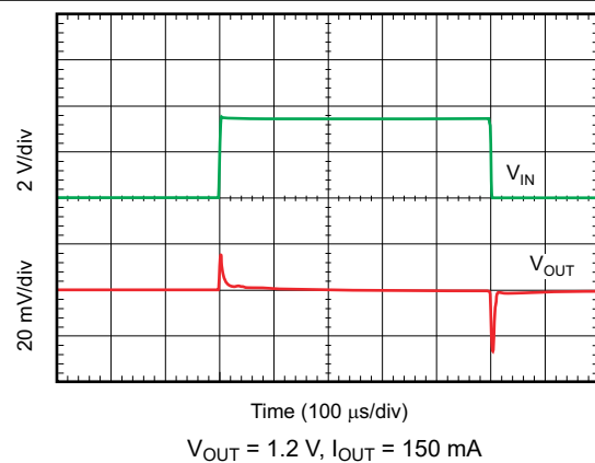
图 8-7. Line Transient Response
