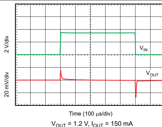
图 6-48. Line Transient Response
