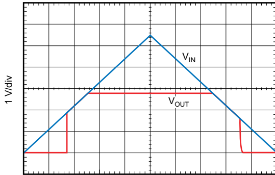
图 6-55. V_{IN} Ramp Up, Ramp Down Response
