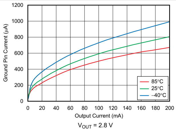
图 6-24. Ground Pin Current vs Output Current
