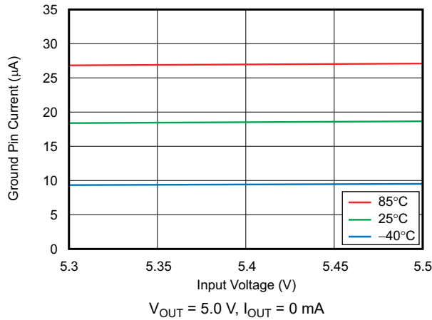
图 6-19. Ground Pin Current vs Input Voltage
