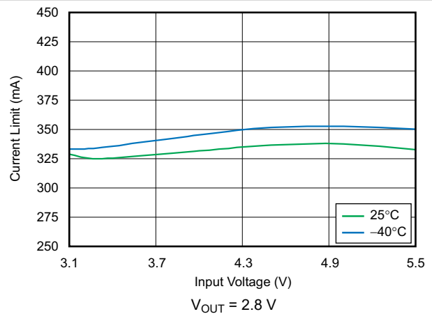
图 6-30. Current Limit vs Input Voltage
