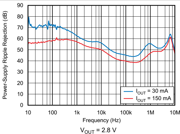
图 6-33. Power-Supply Ripple Rejection vs Frequency
