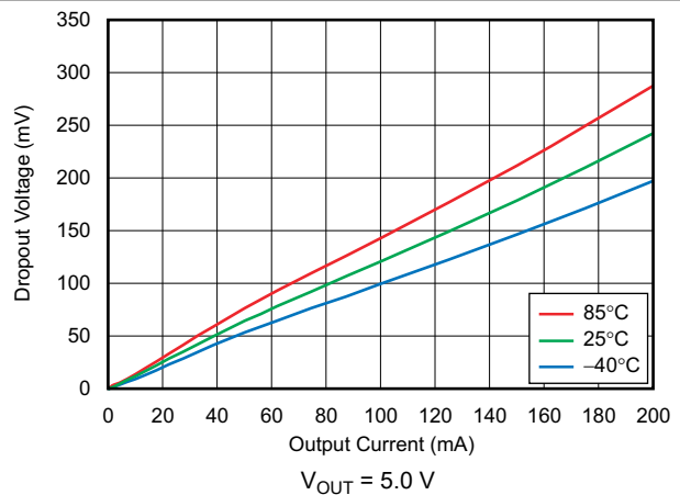
图 6-16. Dropout Voltage vs Output Current
