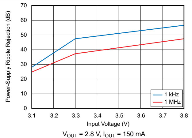
图 6-36. Power-Supply Ripple Rejection vs Input Voltage
