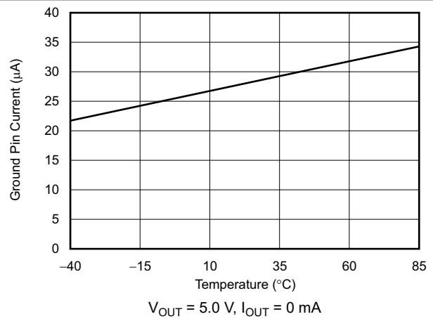
图 6-22. Ground Pin Current vs Temperature
