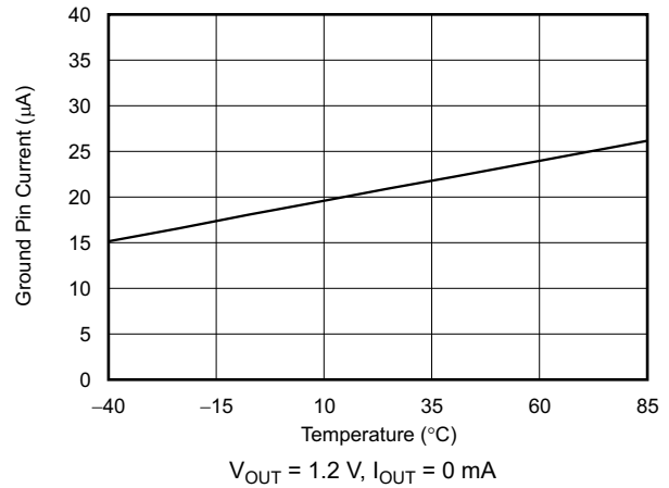
图 6-20. Ground Pin Current vs Temperature
