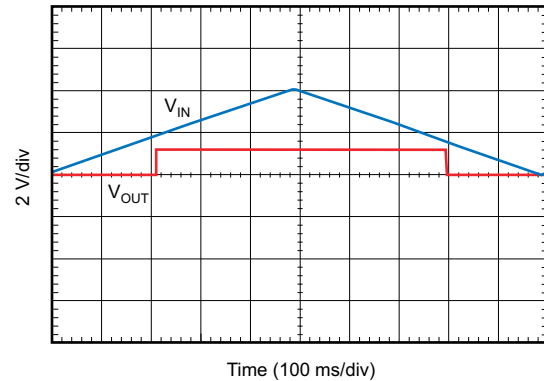
图 8-9. V_{IN} Ramp Up, Ramp Down Response
