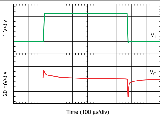
图 6-51. Line Transient Response
