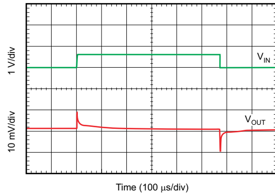
图 6-50. Line Transient Response
