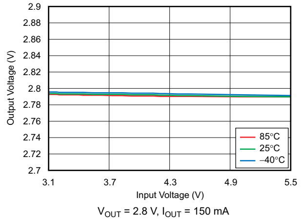
图 6-8. Line Regulation
