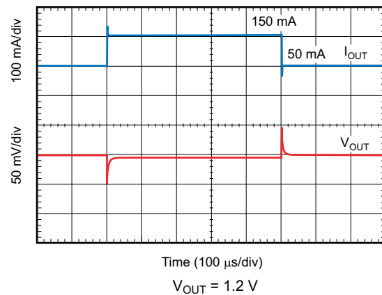
图 6-40. Load Transient Response
