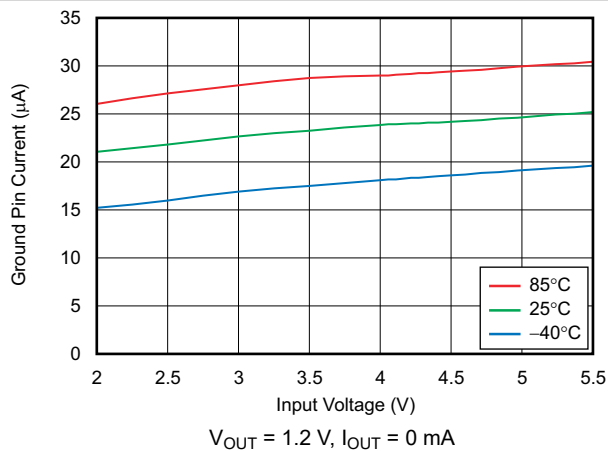
图 6-17. Ground Pin Current vs Input Voltage
