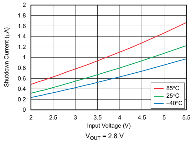
图 6-27. Shutdown Current vs Input Voltage
