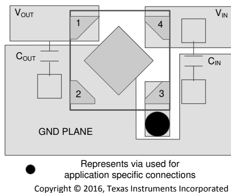
图 8-10. Recommended Layout Example
