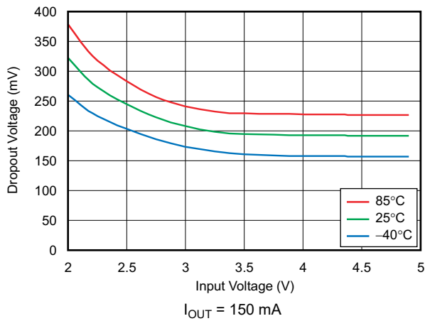
图 6-13. Dropout Voltage vs Input Voltage
