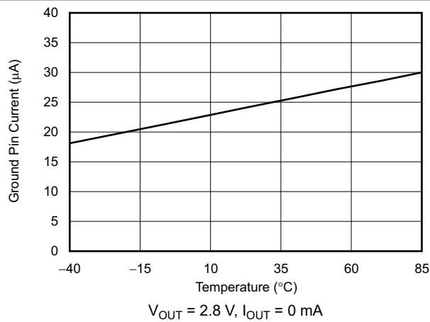
图 6-21. Ground Pin Current vs Temperature
