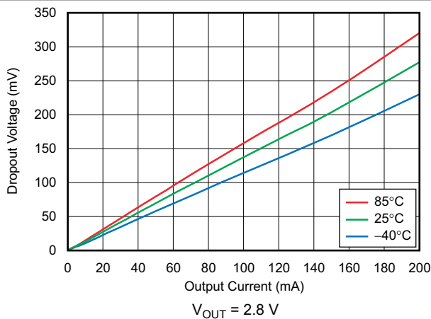
图 6-15. Dropout Voltage vs Output Current
