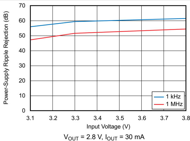
图 6-35. Power-Supply Ripple Rejection vs Input Voltage
