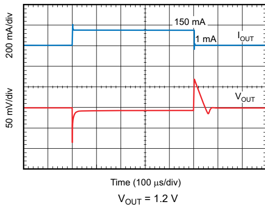
图 6-41. Load Transient Response
