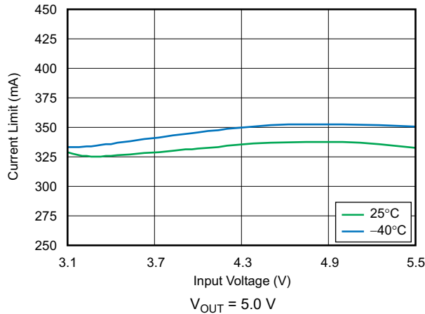
图 6-31. Current Limit vs Input Voltage
