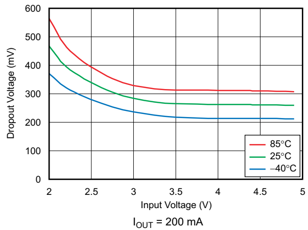
图 6-14. Dropout Voltage vs Input Voltage
