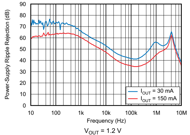
图 6-32. Power-Supply Ripple Rejection vs Frequency
