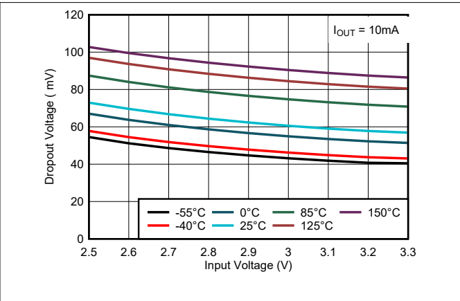
图 6-8. Dropout Voltage vs Input Voltage (TLV70433) for New Chip
