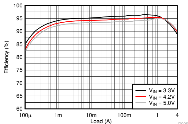
图 8-8. Efficiency
