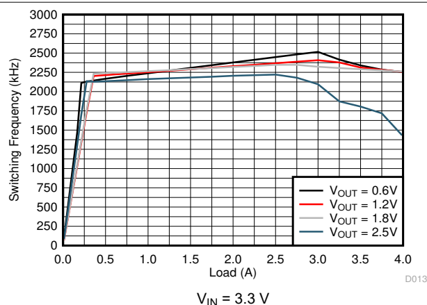
图 8-12. Switching Frequency
