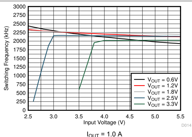
图 8-13. Switching Frequency
