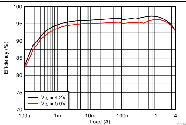
图 8-8. Efficiency
