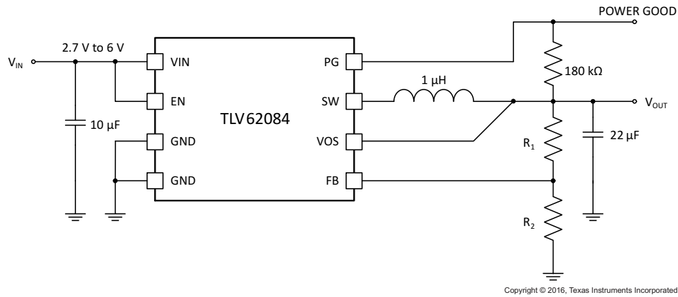
图 10. Typical Application Circuit
