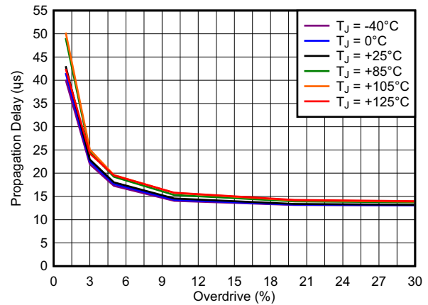
图 6-17. Propagation Delay vs Overdrive ( V+ = 5.5\text{ V} )
