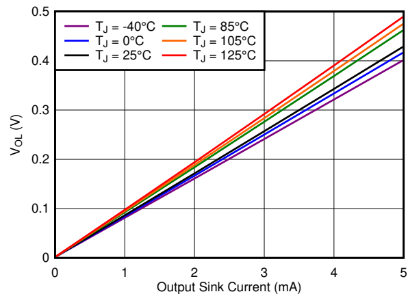
图 6-8. Output Voltage Low vs Output Current ( V_+ = 3.3\text{ V} )
