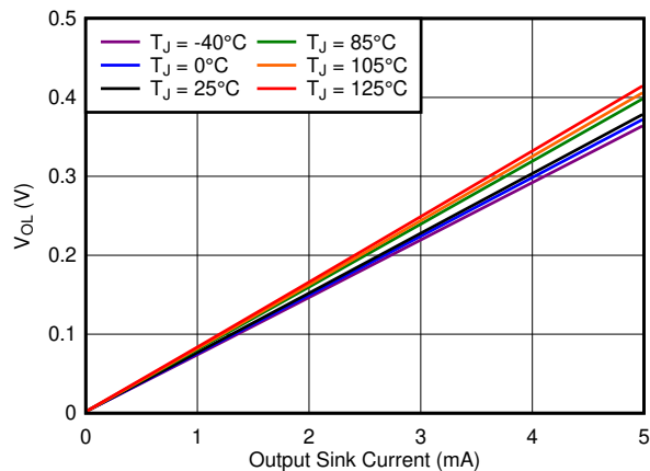
图 6-9. Output Voltage Low vs Output Current ( V_+ = 5.5\text{ V} )
