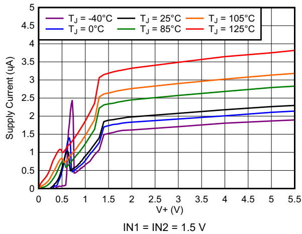
图 6-2. Supply Current vs Supply Voltage
