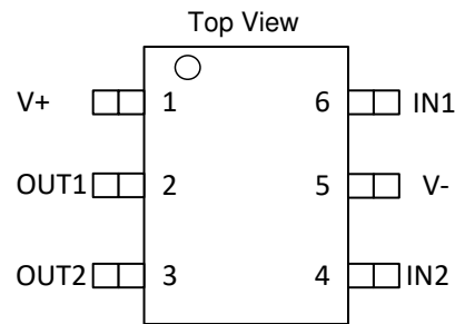
图 5-1. DBV Package, 6-Pin SOT-23
