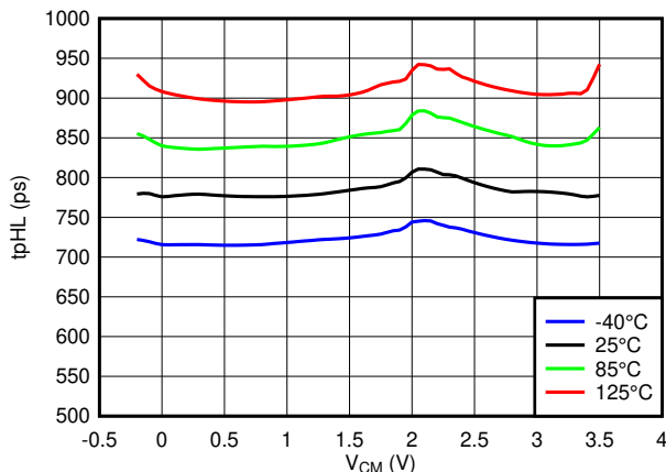
图 5-17. T_{PHL} vs V_{CM} @ V_{CC} = 3.3\text{V}
