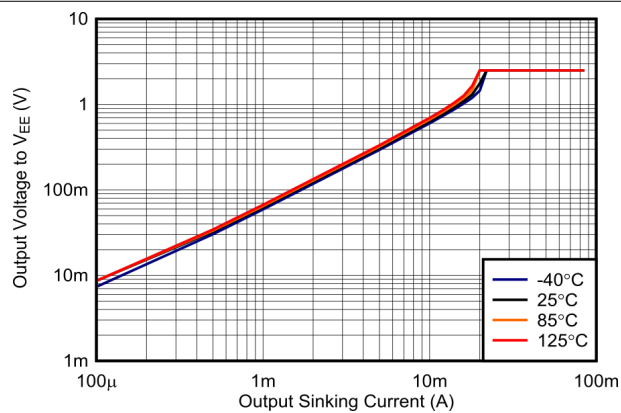
图 6-26. Output Voltage vs. Output Sinking Current, 2.5 V
