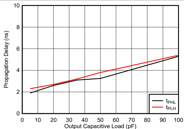
图 6-46. Propagation Delay vs. Load Capacitance, 5 V
