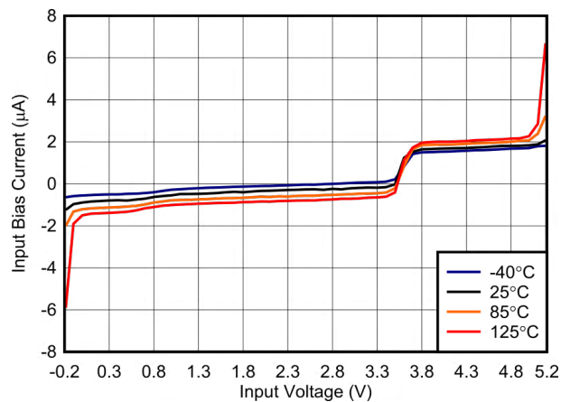
图 6-24. Bias Current vs. Input Voltage, 5 V
