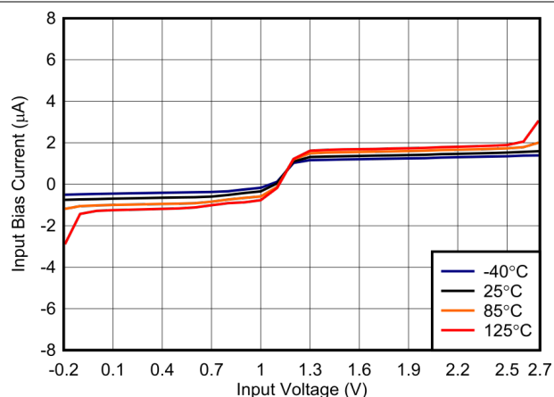
图 6-22. Bias Current vs. Input Voltage, 2.5 V
