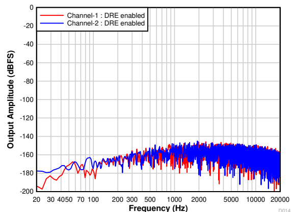
图 7-17. FFT With Idle Input With DRE Enabled
