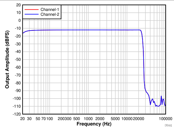
图 7-15. Frequency Response With a -12-dBr Input
