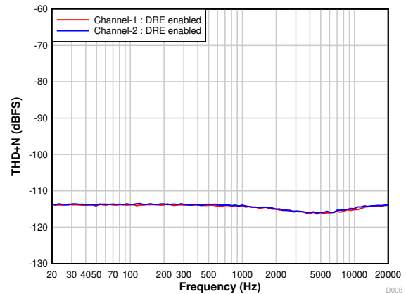
图 7-11. THD+N vs Input Frequency at -60-dBr Input With DRE Disabled
