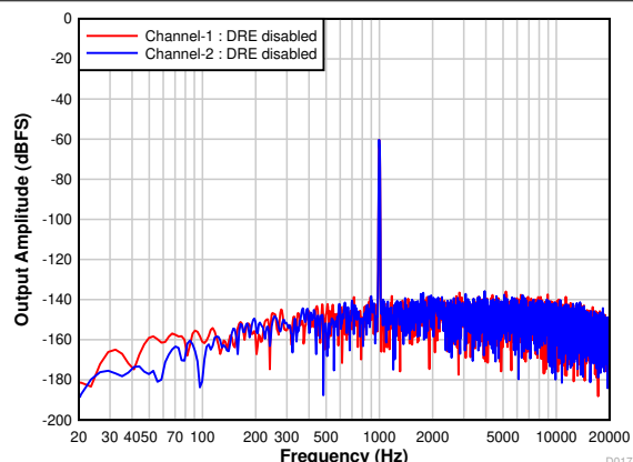
图 7-20. FFT With a -60-dBr Input With DRE Disabled
