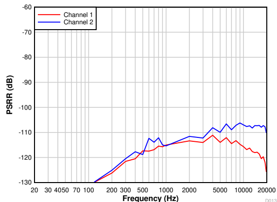
图 7-16. Power-Supply Rejection Ratio vs Ripple Frequency With 100-mV PP Amplitude
