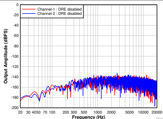
图 7-18. FFT With Idle Input With DRE Disabled
