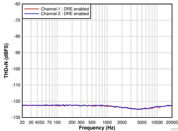
图 7-10. THD+N vs Input Frequency at -60-dBr Input With DRE Enabled
