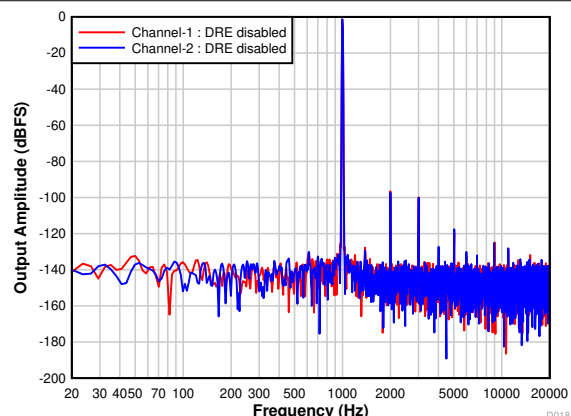
图 7-21. FFT With a -1-dBr Input With DRE Disabled
