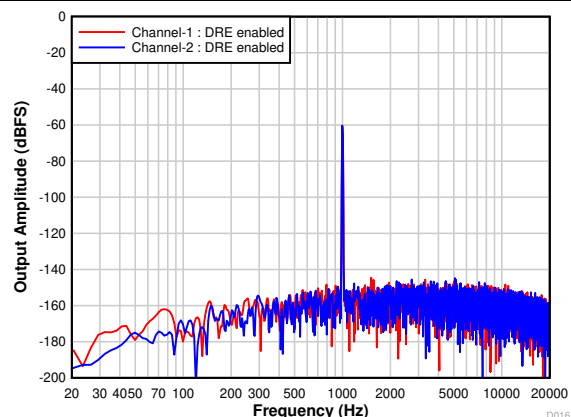
图 7-19. FFT With a -60-dBr Input With DRE Enabled
