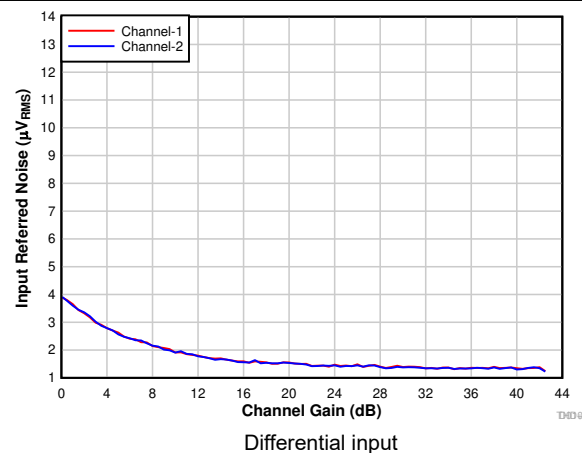
图 7-13. Input-Referred Noise vs Channel Gain
