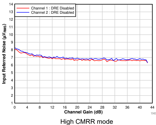
Figure 7-24. Input-Referred Noise vs Channel Gain
