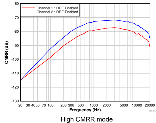
Figure 7-23. Common-Mode Rejection Ratio vs Ripple Frequency With 100-mV pp Amplitude and DRE Enabled
