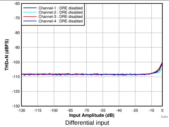
图 6. THD+N vs Input Amplitude With DRE Disabled
