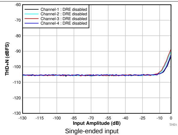
图 8. THD+N vs Input Amplitude With DRE Disabled
