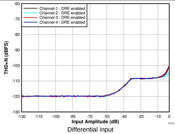
图 5. THD+N vs Input Amplitude With DRE Enabled
