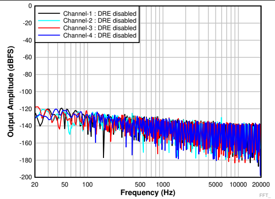
图 18. FFT With Idle Input With DRE Disabled
