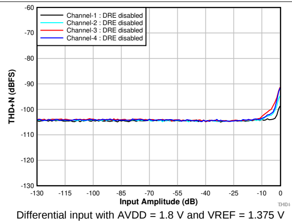
图 10. THD+N vs Input Amplitude With DRE Disabled
