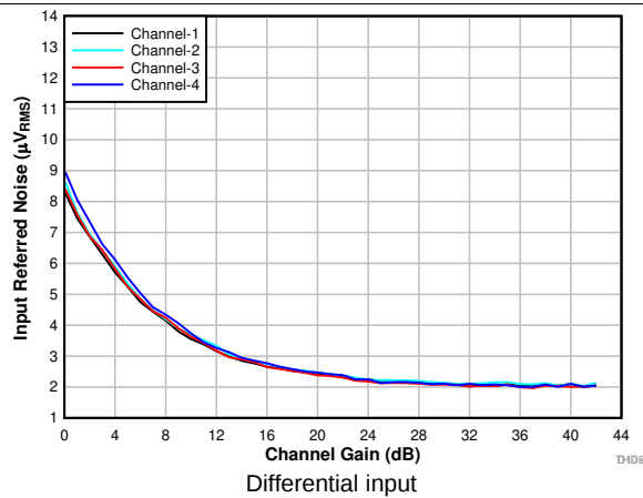
图 13. Input-Referred Noise vs Channel Gain Differential input
