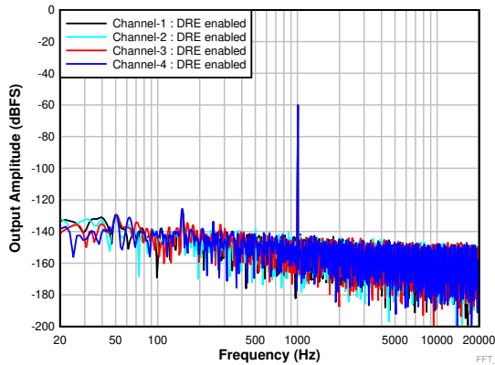
图 17. FFT With Idle Input With DRE Enabled
