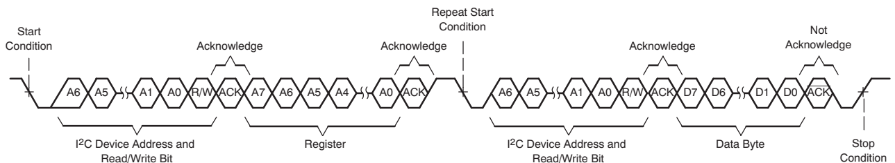
图 91. I 2 C Single-Byte Read Transfer
