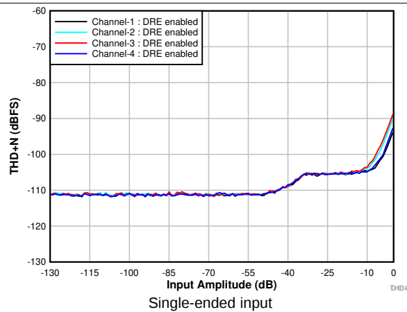
图 7. THD+N vs Input Amplitude With DRE Enabled
