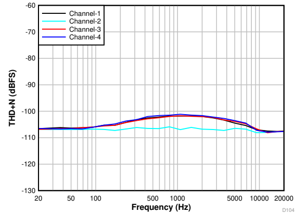
图 12. THD+N vs Input Frequency With a -1\text{-dBr} Input
