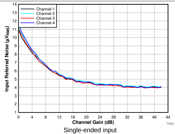
图 14. Input-Referred Noise vs Channel Gain Single-ended input
