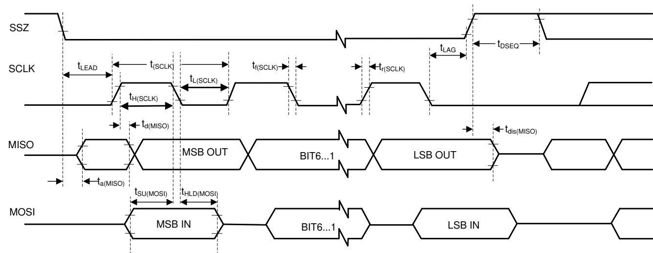
图 2. SPI Interface Timing Diagram
