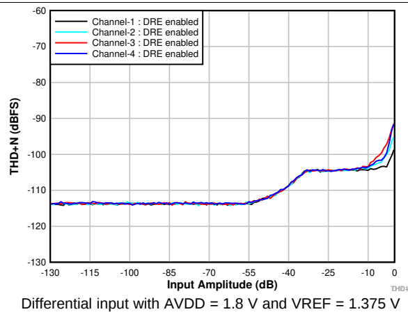
图 9. THD+N vs Input Amplitude With DRE Enabled
