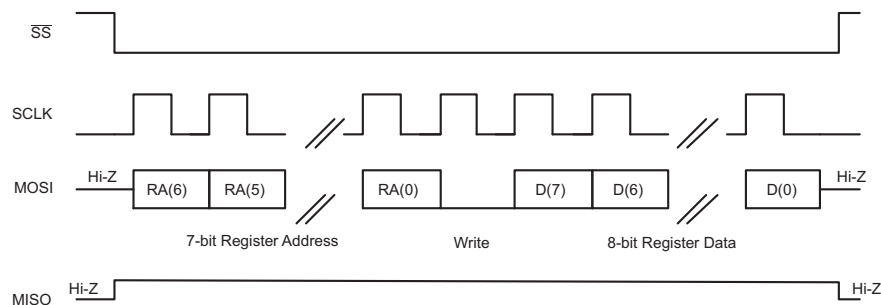
图 93. SPI Single-Byte Write Transfer
