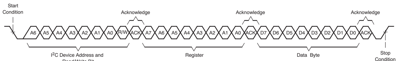
图 89. I²C Single-Byte Write Transfer
