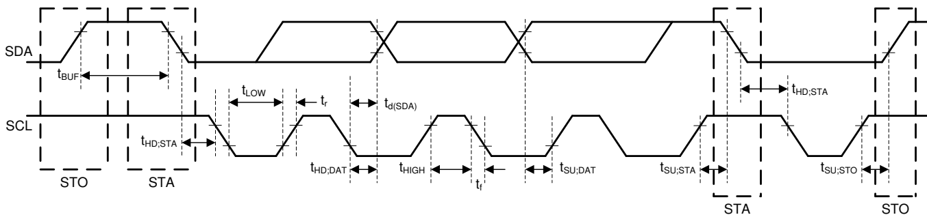
图 1. I²C Interface Timing Diagram
