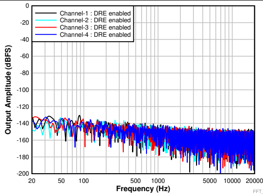
图 17. FFT With Idle Input With DRE Enabled
