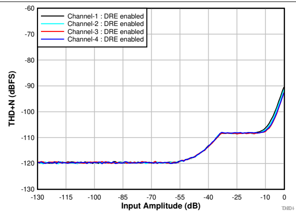
图 174. THD+N vs Input Amplitude With DRE Enabled
