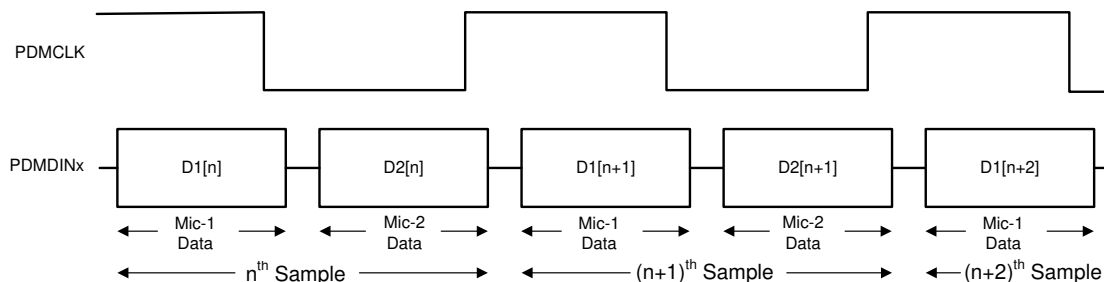
图 87. Digital PDM Microphone Protocol Timing Diagram
