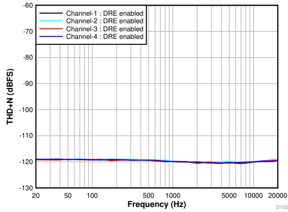
图 11. THD+N vs Input Frequency With a -60\text{-dBr} Input
