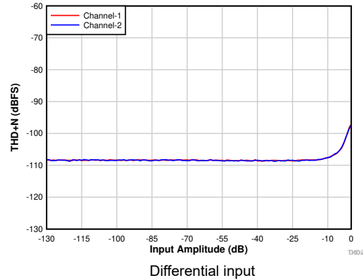
图 7-5. THD+N vs Input Amplitude With DRE Disabled
