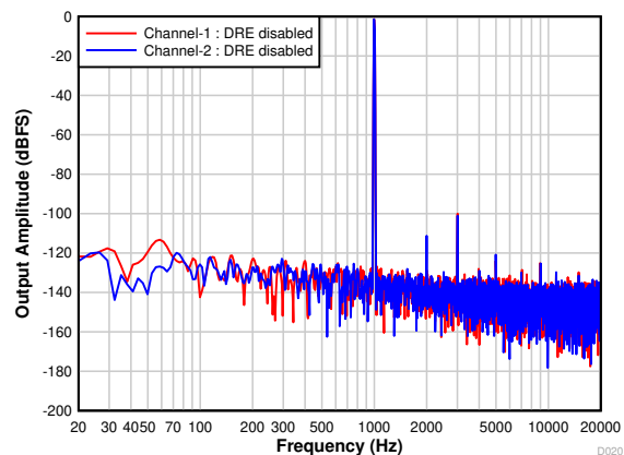
图 7-23. FFT With a -1-dBr Input With DRE Disabled
