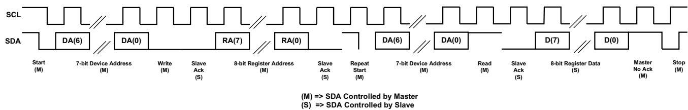
Figure 13. I²C Read
