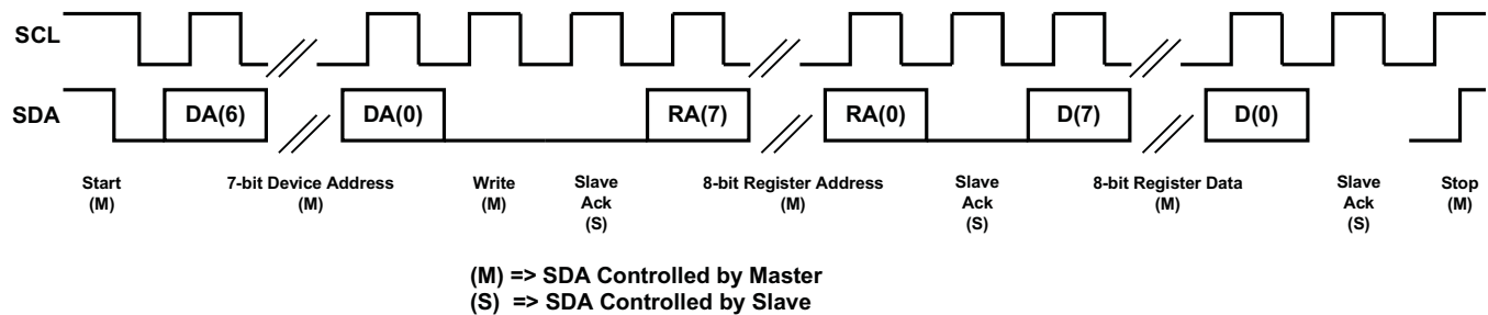
Figure 12. I²C Write
