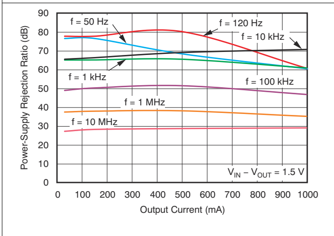
图 6-11. Power-Supply Rejection Ratio vs Output Current
