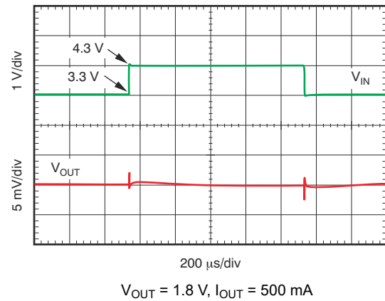
图 6-22. Line Transient Response
