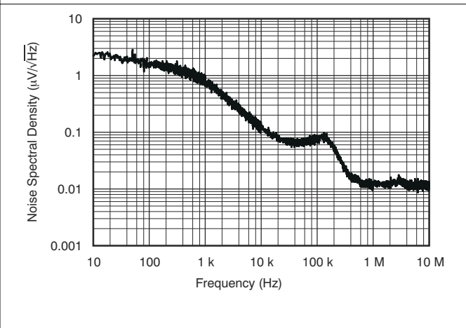
图 6-12. Spectral Noise Density vs Frequency
