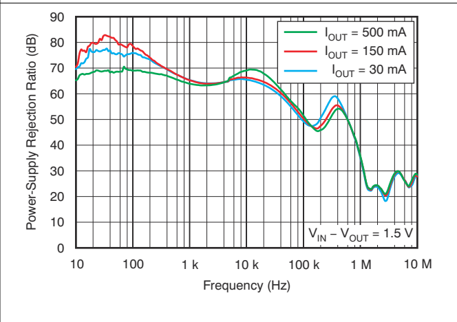
图 6-10. Power-Supply Rejection Ratio vs Frequency
