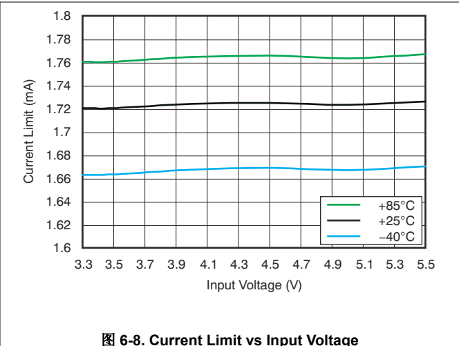
图 6-8. Current Limit vs Input Voltage
