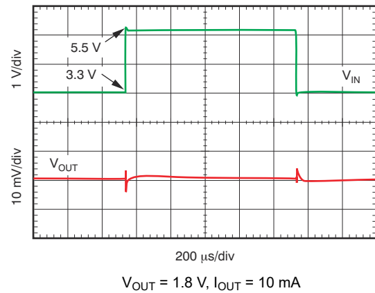
图 6-24. Line Transient Response
