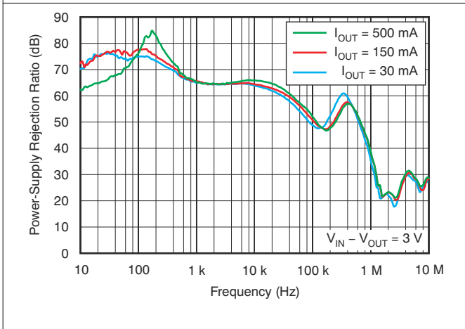
图 6-9. Power-Supply Rejection Ratio vs Frequency
