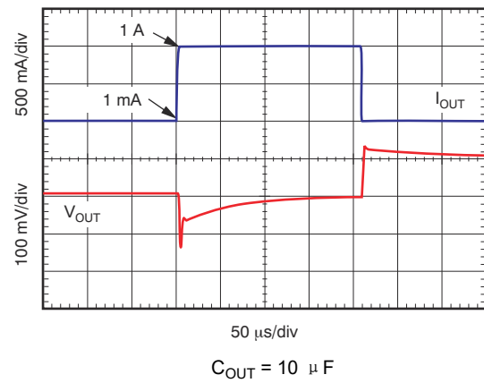
图 6-20. Load Transient Response 1 mA to 1 A
