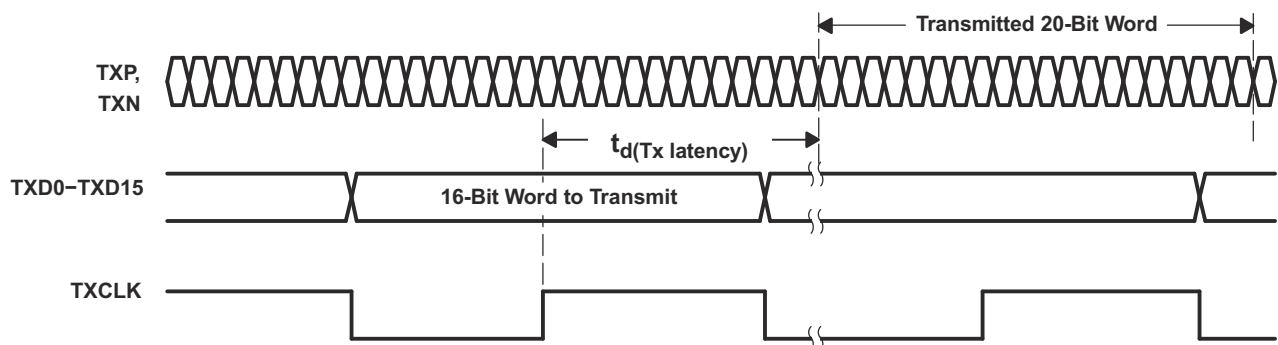
图 6-2. Transmitter Latency
