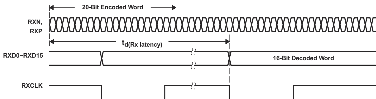
图 6-5. Receiver Latency
