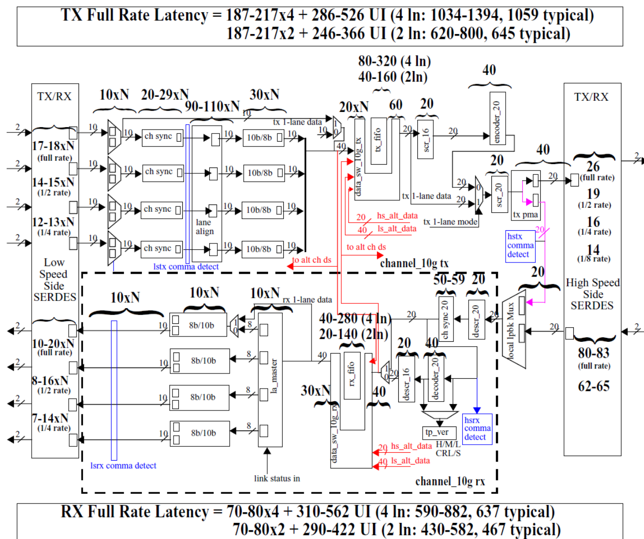
Figure 7-13. General Purpose SERDES Mode Latency
