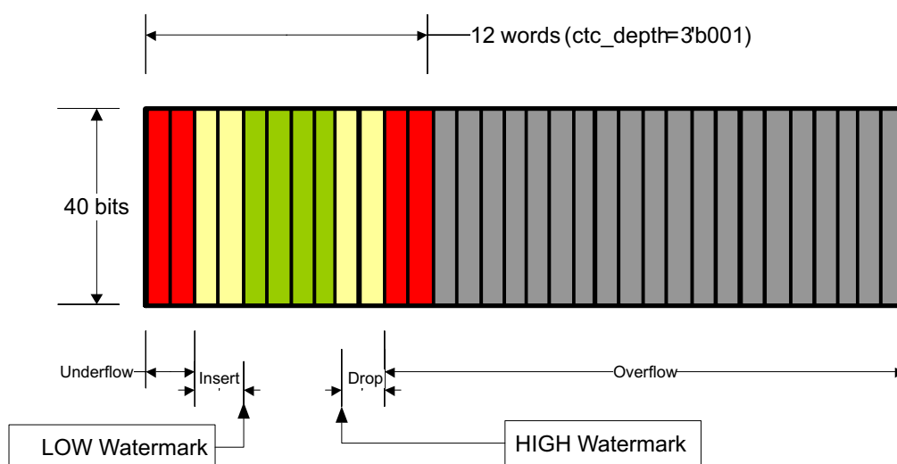
Figure 7-39. Organization of the XAUI CTC FIFO (12-Deep)
