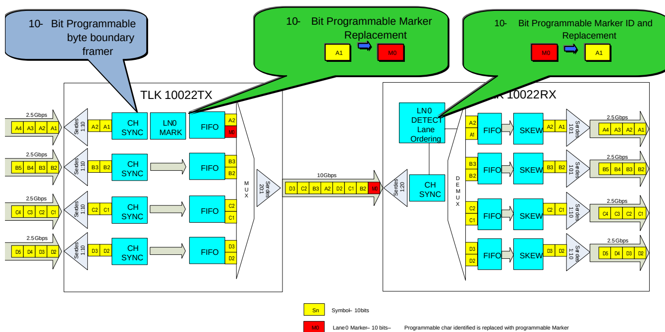
Figure 3-3. Block Diagram of the Interleave/De-Interleave Scheme
