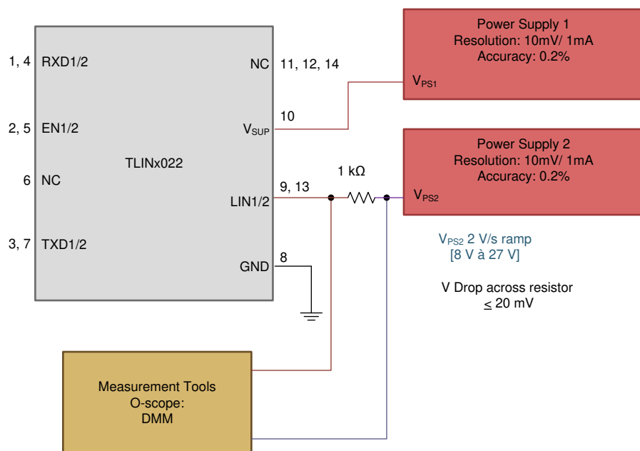
图 7-8. Test Circuit for I_{\text{BUS\_PAS\_rec}} Param 14
