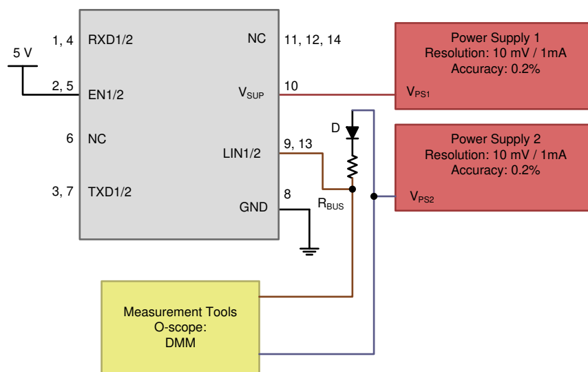
图 7-4. LIN Receiver Test with RX access Parameters 17, 18, 19, 20
