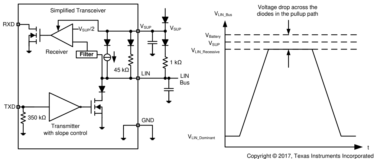
图 7-1. Commander Node Configuration with Voltage Levels
