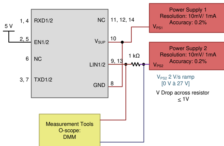
图 7-8. Test Circuit for I_{\text{BUS\_PAS\_rec}} Param 14
