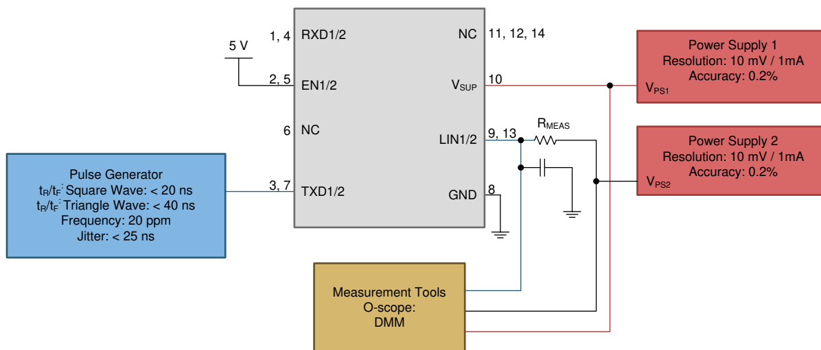
图 7-10. Test Circuit for I_{BUS\_NO\_BAT} Loss of Battery
