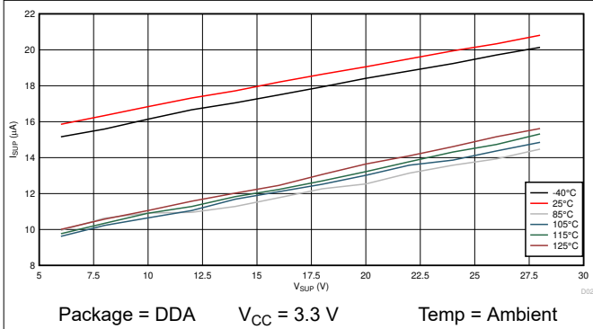
图 7-9. Sleep Mode Current Across V_{SUP} and Temperature
