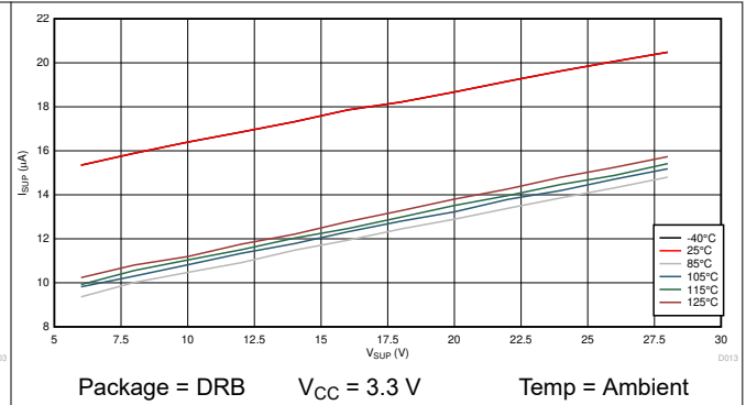
图 7-8. Sleep Mode Current Across V_{SUP} and Temperature
