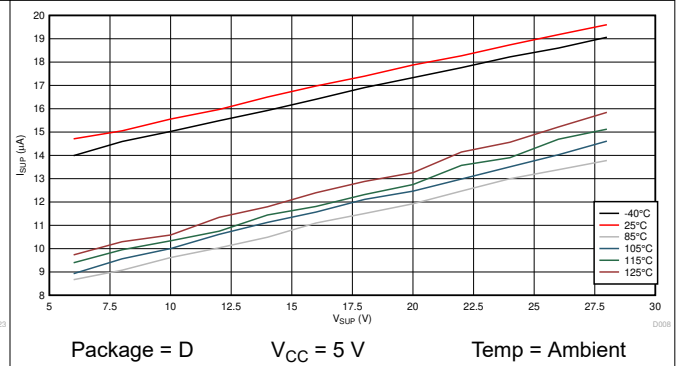
图 7-10. Sleep Mode Current Across V_{SUP} and Temperature
