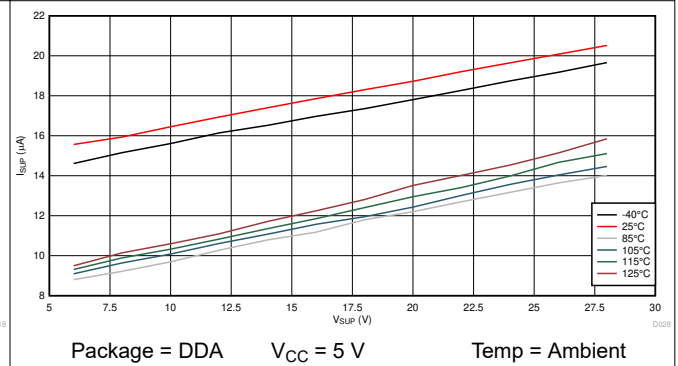
图 7-12. Sleep Mode Current Across V_{SUP} and Temperature
