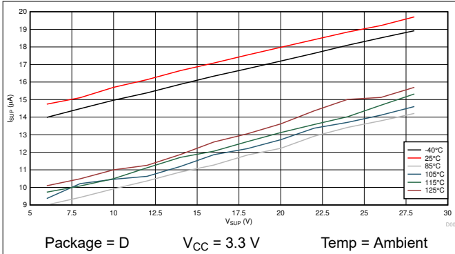
图 7-7. Sleep Mode Current Across V_{SUP} and Temperature
