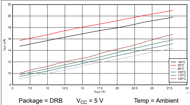
图 7-11. Sleep Mode Current Across V_{SUP} and Temperature
