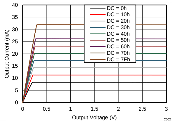
Figure 2. Output Current vs Output Voltage (DCX n Changing)
