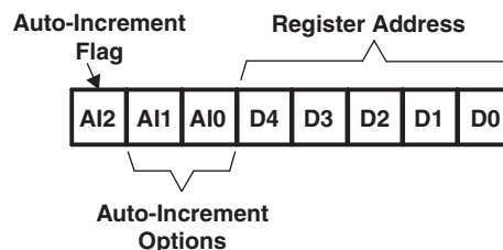
Figure 21. Control Register
