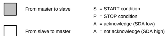
图 24. Legend for the I 2 C Sequence Diagrams
