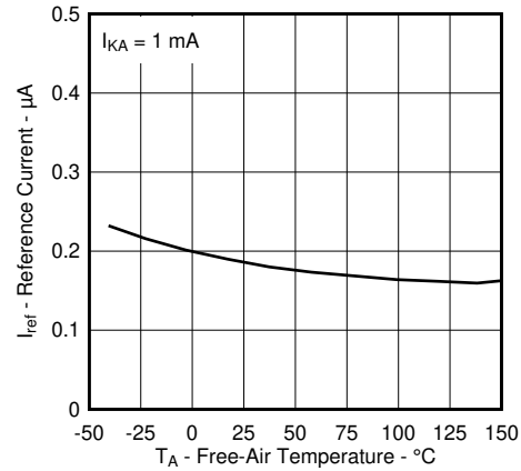
图 2. Reference Current versus Free-Air Temperature
