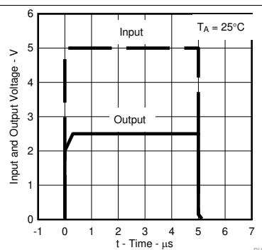
图 10. Pulse Response
