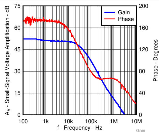
图 6. Small-Signal Voltage Amplification versus Frequency
