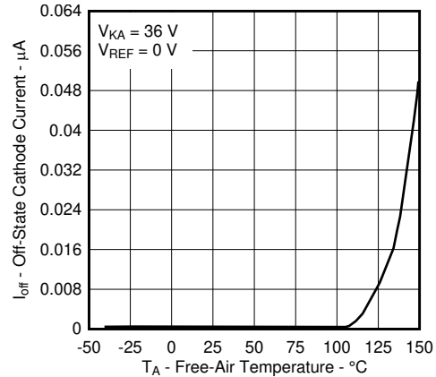
图 4. Off-State Cathode Current versus Free-Air Temperature
