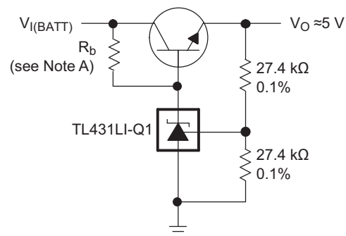
图 32. Efficient 5-V Low-Dropout (LDO) Regulator Configuration
