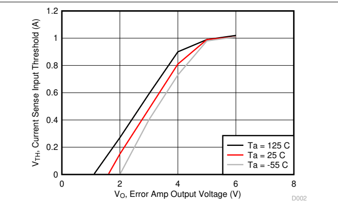
图 5-2. Current Sense Input Threshold vs Error Amplifier Output Voltage for V_{IN} = 15\text{ V}
