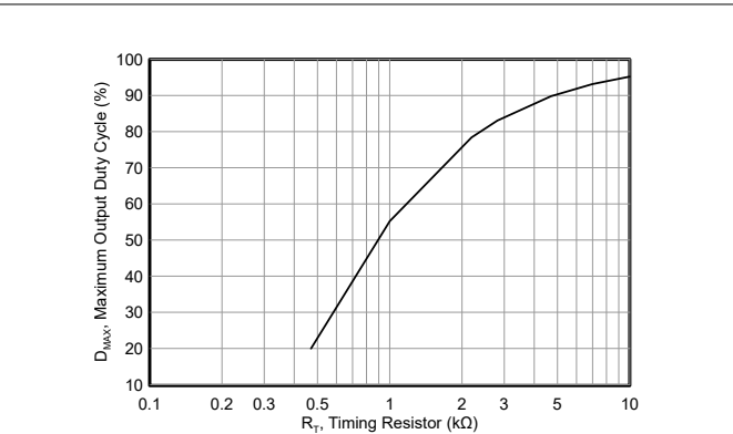
图 5-4. Max Output Duty Cycle vs Timing Resistor for V_{CC} = 15 , C_T = 3.3\text{ nF} , T_A = 25^\circ\text{C}
