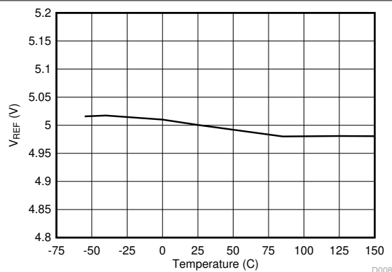
图 5-8. Reference Voltage vs Temperature
