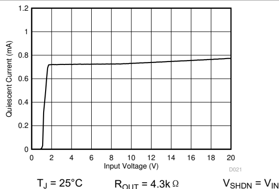
T_J = 25^\circ\text{C} R_{OUT} = 4.3\text{k}\Omega V_{SHDN} = V_{IN}
