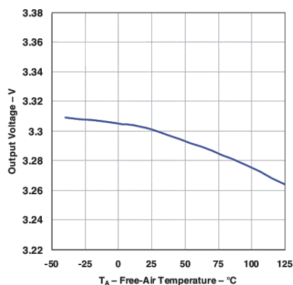
I_{OUT} = 1\text{mA} TL1963A-33
