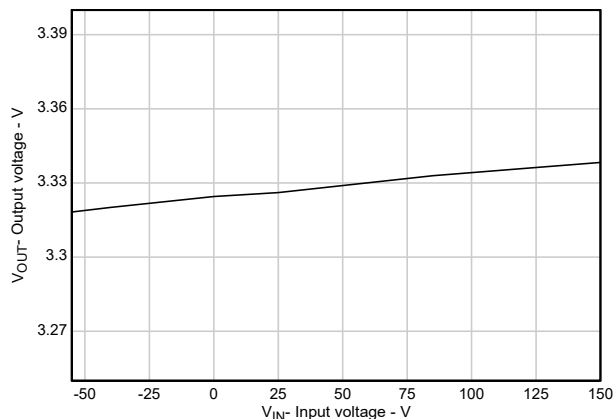
I_{OUT} = 1\text{mA} TL1963A-33
