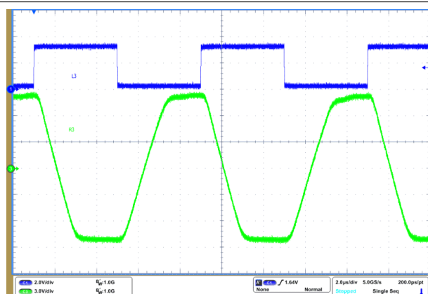
V_{CC} = 5V 总线负载 = 5k\Omega \parallel 2.5nF 250kbps SLR = V_{IO}
