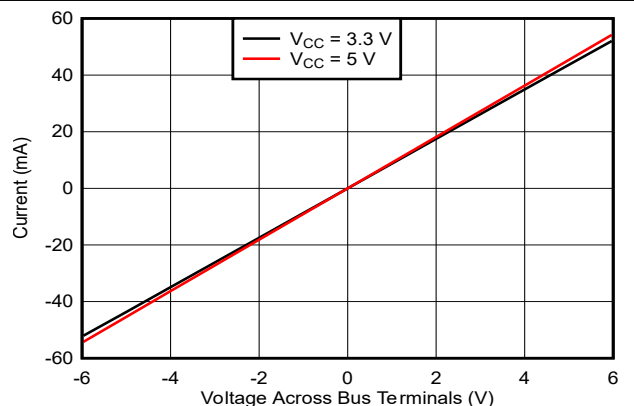
TERM_TX = V_{IO}
