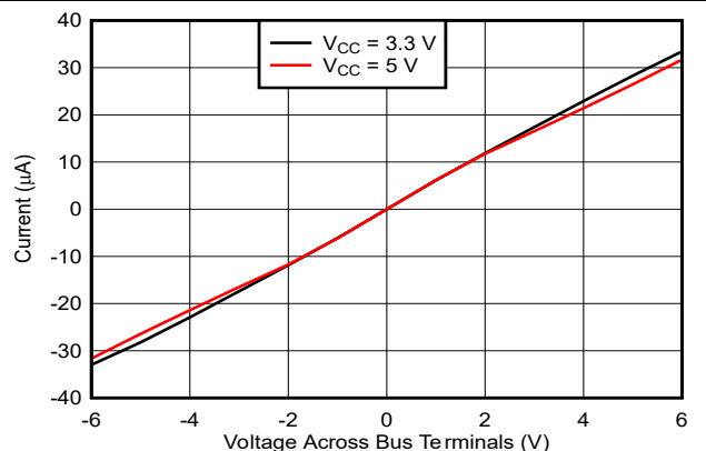
TERM_TX = GND
