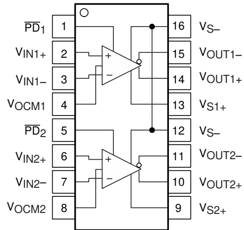
图 5-2. PW Package 16-Pin VSSOP Top View
