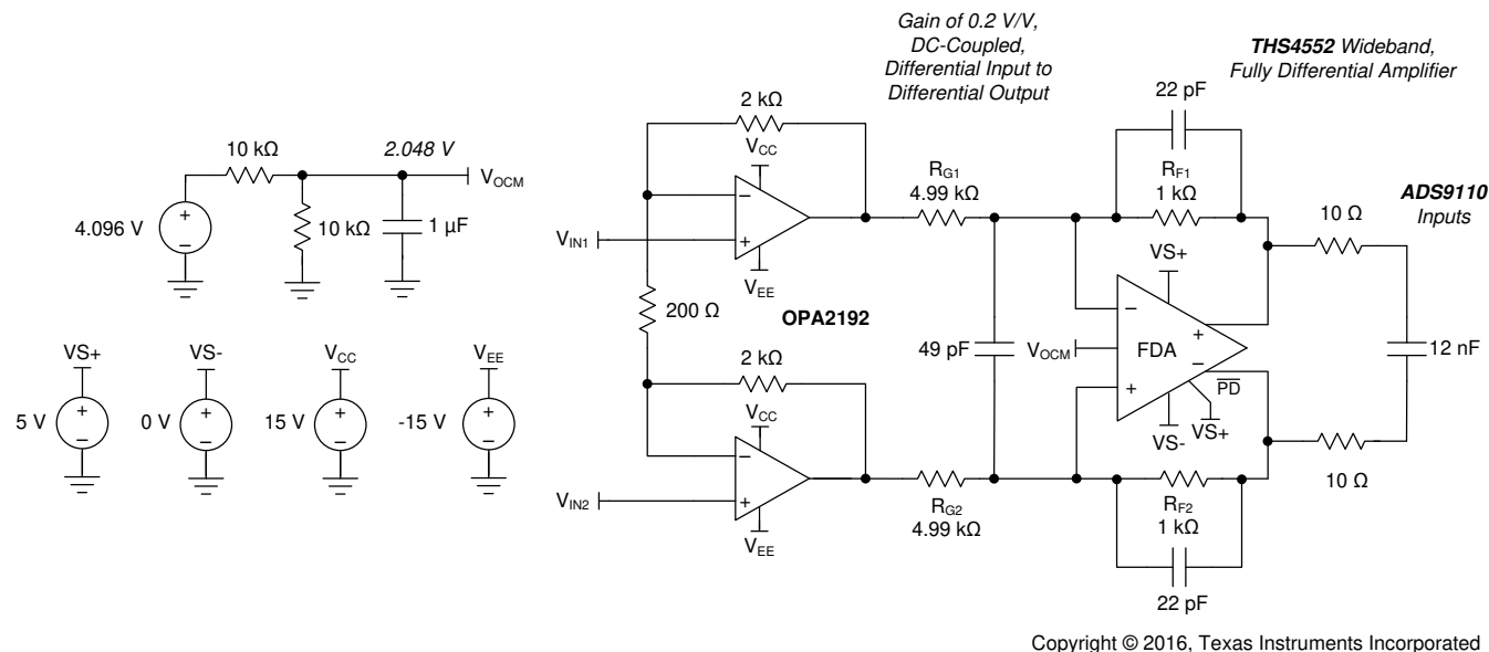
图 8-11. Example DC-Coupled Differential I/O Design from a Precision Dual Op Amp to an 18-Bit SAR
