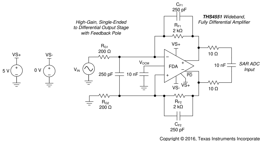
图 10-9. Single-Ended to Differential Stage with a Feedback Pole and Differential Input Capacitor
