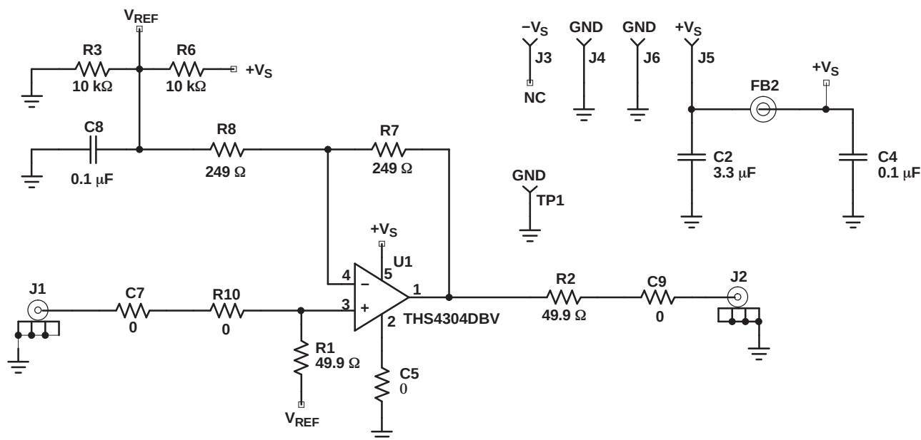
Figure 44. Non-Inverting 5-V Single-Supply Amplifier
