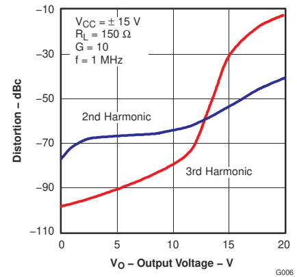
图 5-35. Distortion vs Output Voltage
