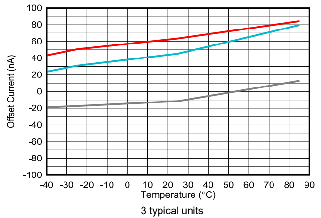
图 5-26. Input Offset Current vs Ambient Temperature
