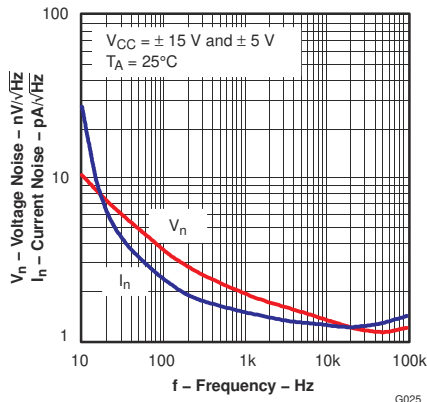
图 5-54. Voltage and Current Noise vs Frequency
