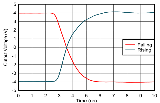
图 7-18. Settling Time
