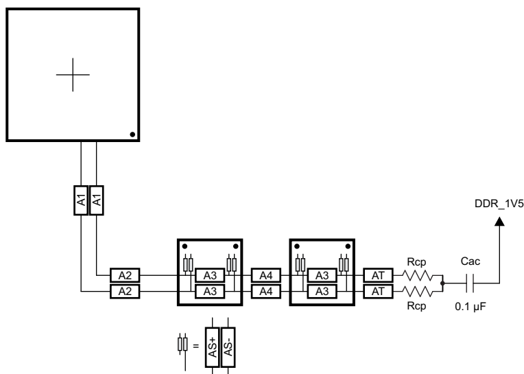
图 7-63. CK Routing for Four Mirrored DDR3 Devices
