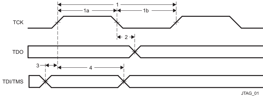
图 5-101. JTAG Timing
