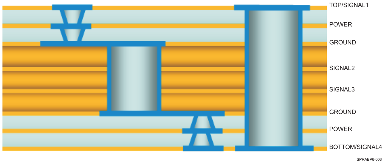
图 7-3. Layer PCB With Plated Through Holes (PTH) Vias
