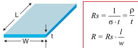
图 7-9. Depiction of Sheet Resistivity and Resistance
