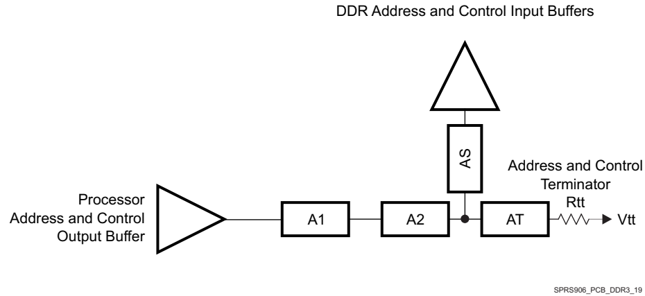
图 7-72. ADDR_CTRL Topology for One DDR3 Device
