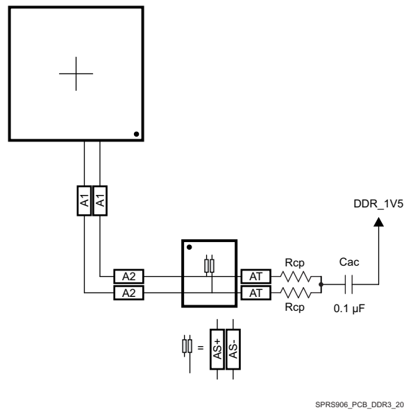
图 7-73. CK Routing for One DDR3 Device
