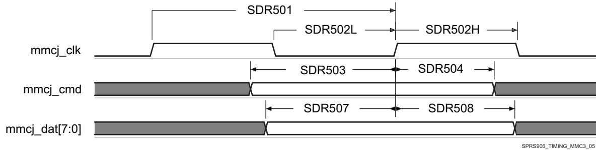
图 5-99. MMC/SD/SDIOj in - High Speed SDR50 - Receiver Mode
