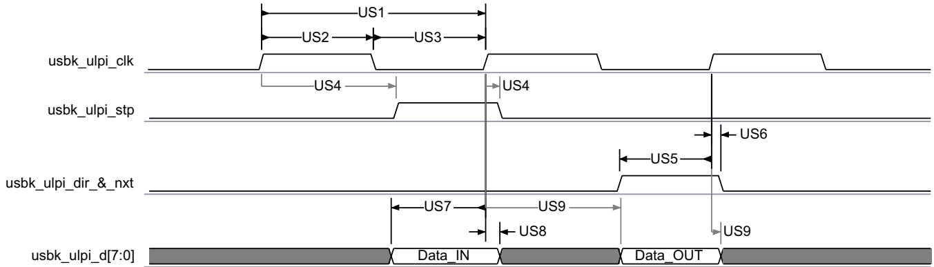
图 5-60. HS USB3 ULPI —SDR—Slave Mode—12-pin Mode
