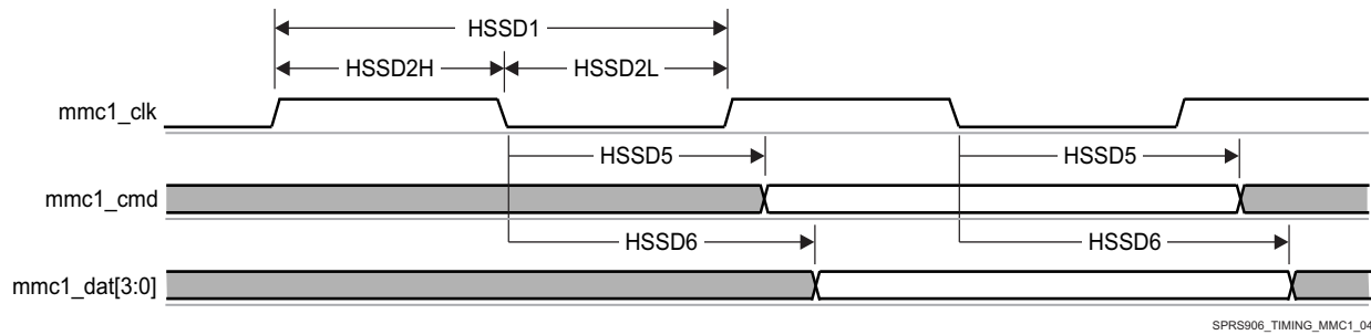
图 5-73. MMC/SD/SDIO in - High Speed - Transmitter Mode
