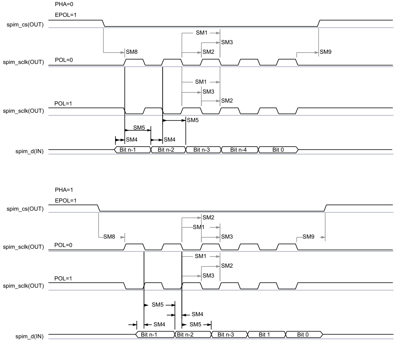
图 5-43. McSPI - Master Mode Receive
