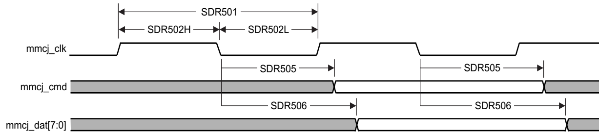
图 5-100. MMC/SD/SDIOj in - High Speed SDR50 - Transmitter Mode
