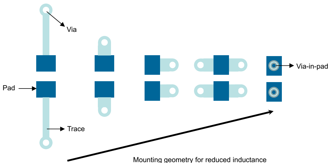
图 7-9. Capacitor Placement Geometry for Improved Mounting Inductance
