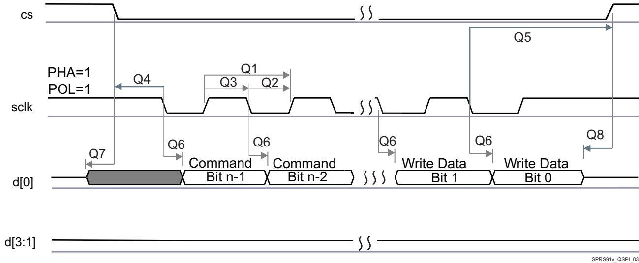
图 5-48. QSPI Write (Clock Mode 3)
