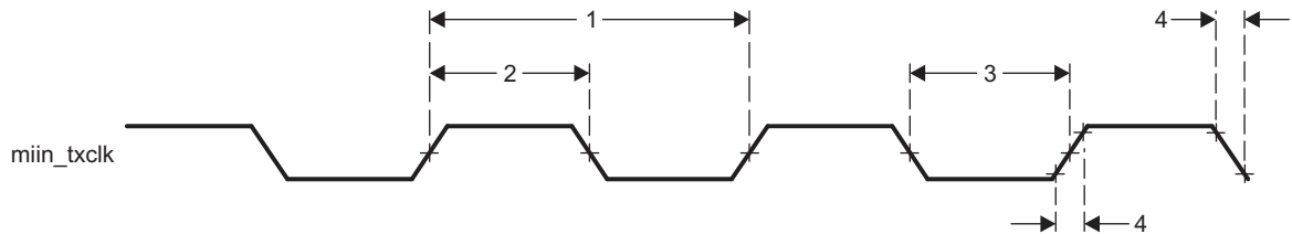
图 5-62. Clock Timing (GMAC Transmit) - MII operation
