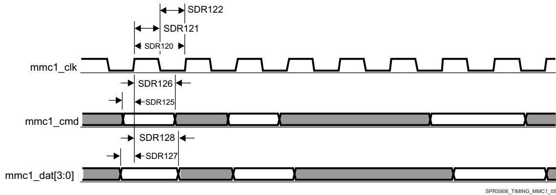
图 5-74. MMC/SD/SDIO in - High Speed SDR12 - Receiver Mode
