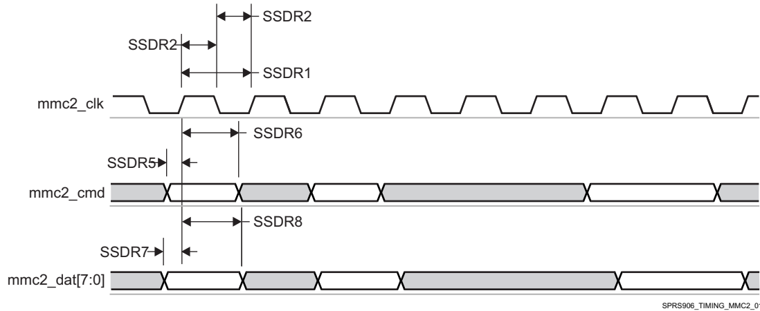
图 5-84. MMC/SD/SDIO in - Standard JC64 - Receiver Mode
