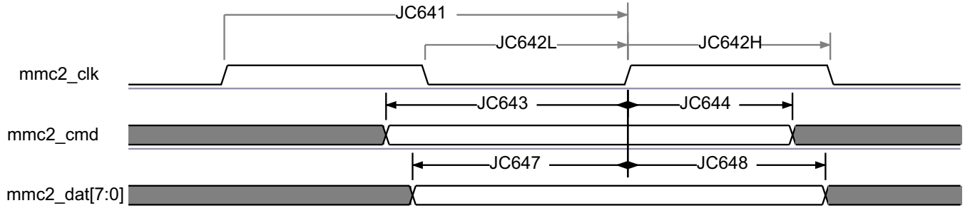
图 5-86. MMC/SD/SDIO in - High Speed JC64 - Receiver Mode
