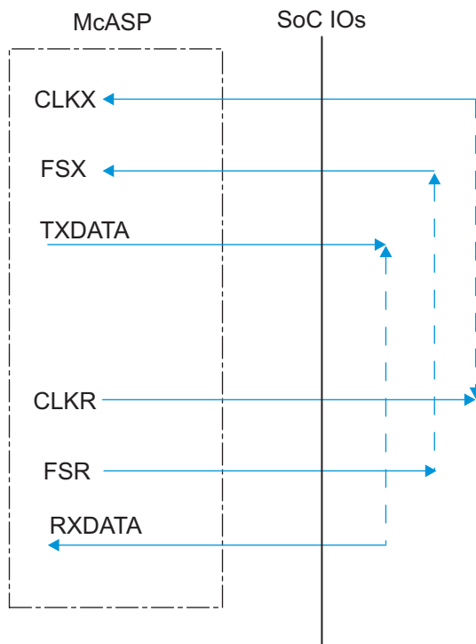
图 5-54. McASP1-8 CIOFIO – ASYNC Mode
