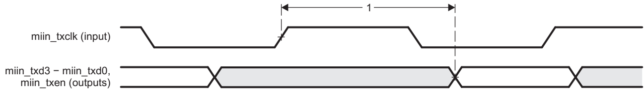
图 5-64. GMAC Transmit Interface Timing MIIn operation
