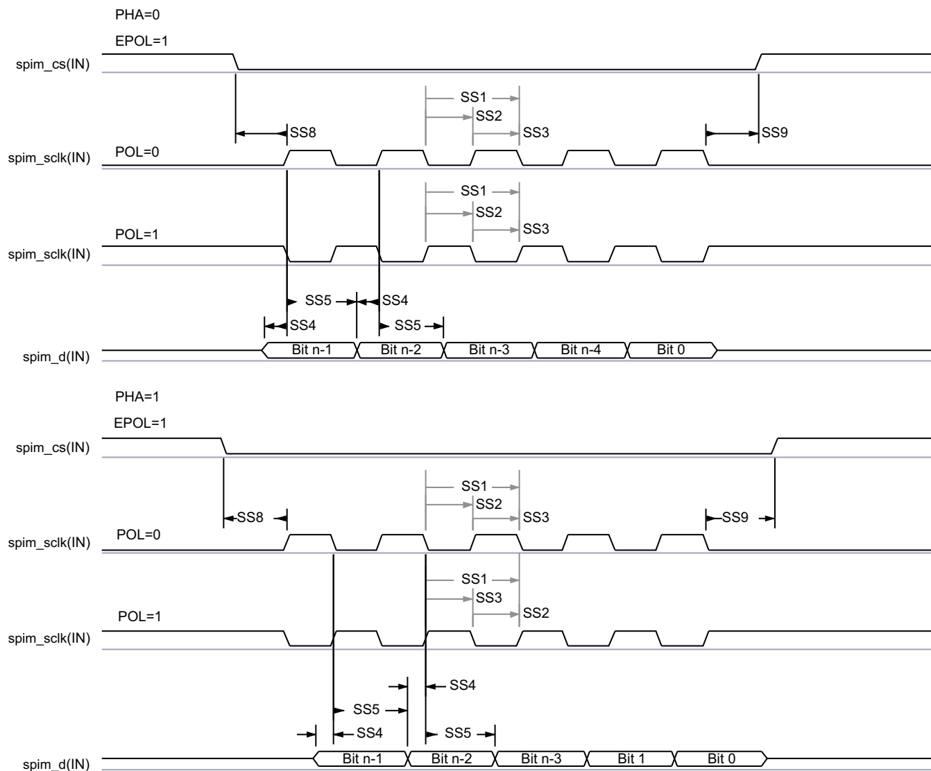
图 5-45. McSPI - Slave Mode Receive
