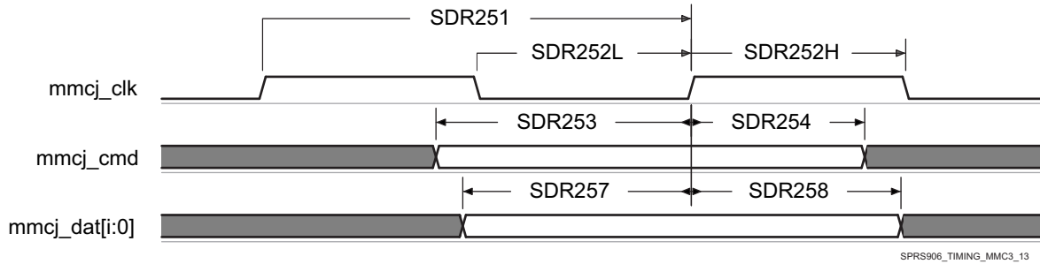
图 5-97. MMC/SD/SDIOj in - SDR25 - Receiver Mode
