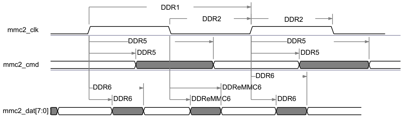
图 5-90. MMC/SD/SDIO in - High Speed DDR JC64 - Transmitter Mode
