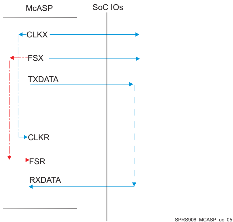
图 5-56. McASP1-8 CO-FO- – SYNC Mode
