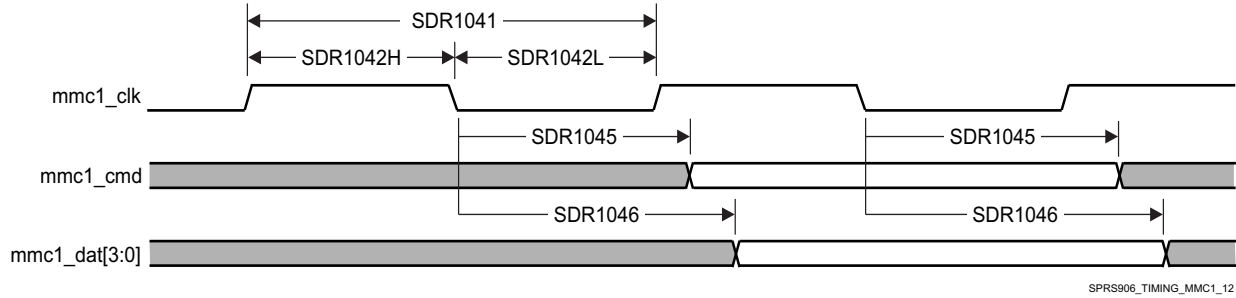
图 5-81. MMC/SD/SDIO in - High Speed SDR104 - Transmitter Mode
