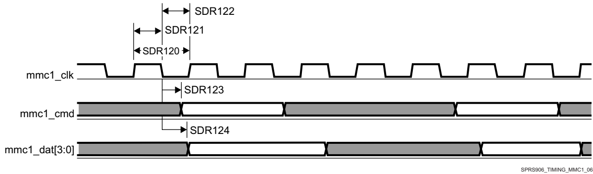
图 5-75. MMC/SD/SDIO in - High Speed SDR12 - Transmitter Mode
