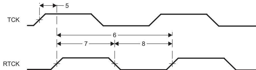
图 5-102. JTAG With RTCK Timing
