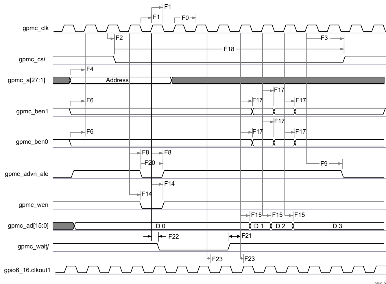
图 5-28. GPMC / Nonmultiplexed 16bits NOR Flash - Synchronous Burst Write 4x16bits - (GpmcFCLKDivider = 0) (1)(2)
