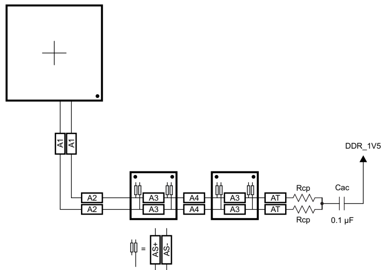
图 7-46. CK Routing for Four Mirrored DDR3 Devices
