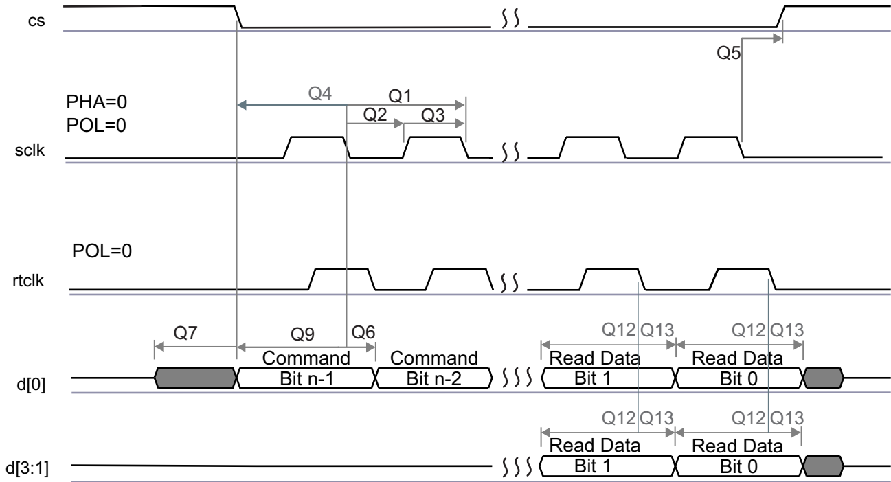
图 5-47. QSPI Read (Clock Mode 0)
