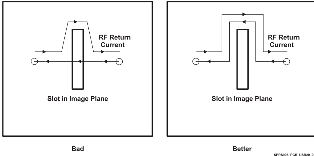
图 7-29. Do Not Violate Image Planes
