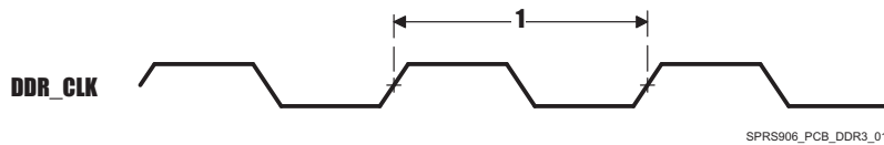
图 7-37. DDR3 Memory Controller Clock Timing
