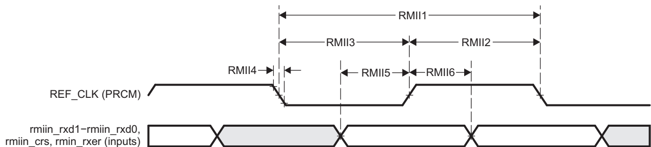
图 5-66. GMAC Receive Interface Timing RMIIIn operation
