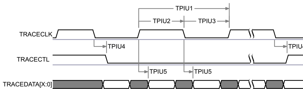
图 5-103. TPIU—PLL DDR Transmit Mode (1)
