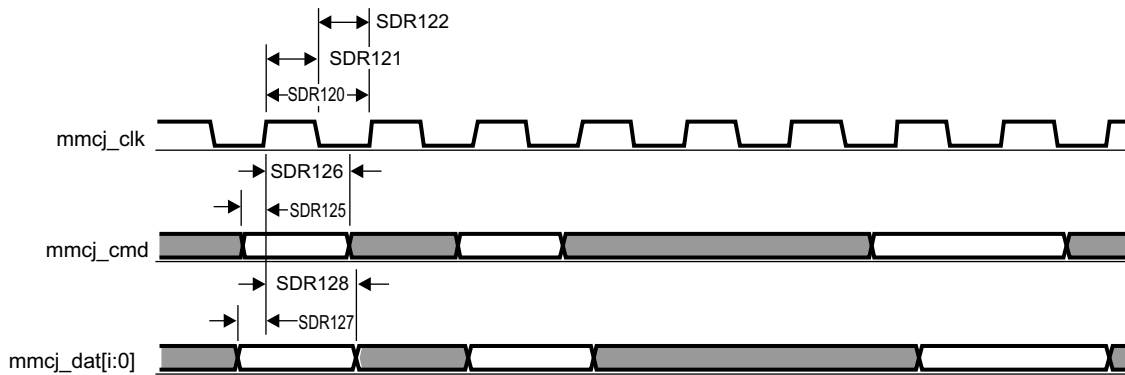
图 5-95. MMC/SD/SDIOj in - SDR12 - Receiver Mode
