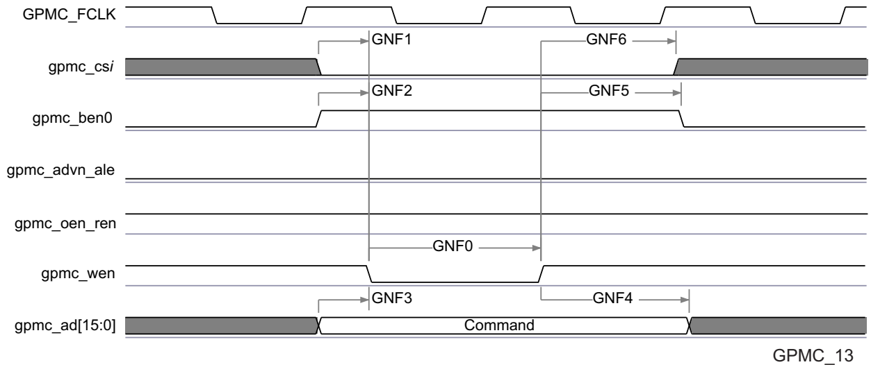
图 5-35. GPMC / NAND Flash - Command Latch Cycle Timing (1)
