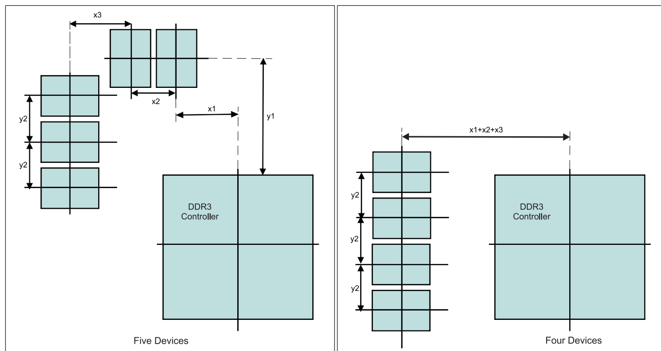
图 7-40. Placement Specifications
