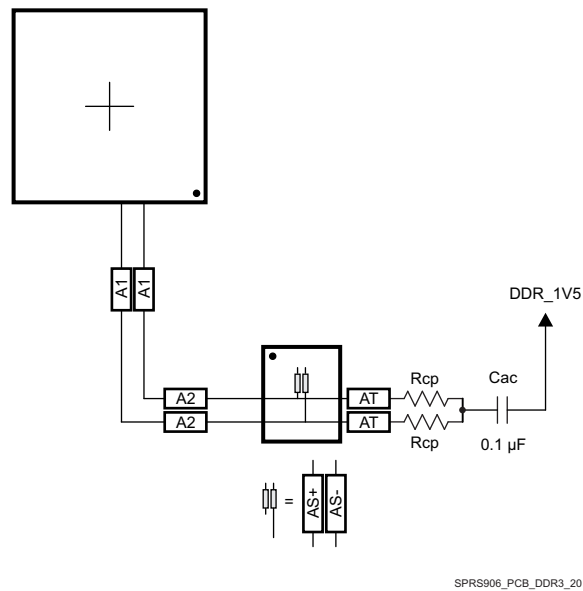
图 7-56. CK Routing for One DDR3 Device
