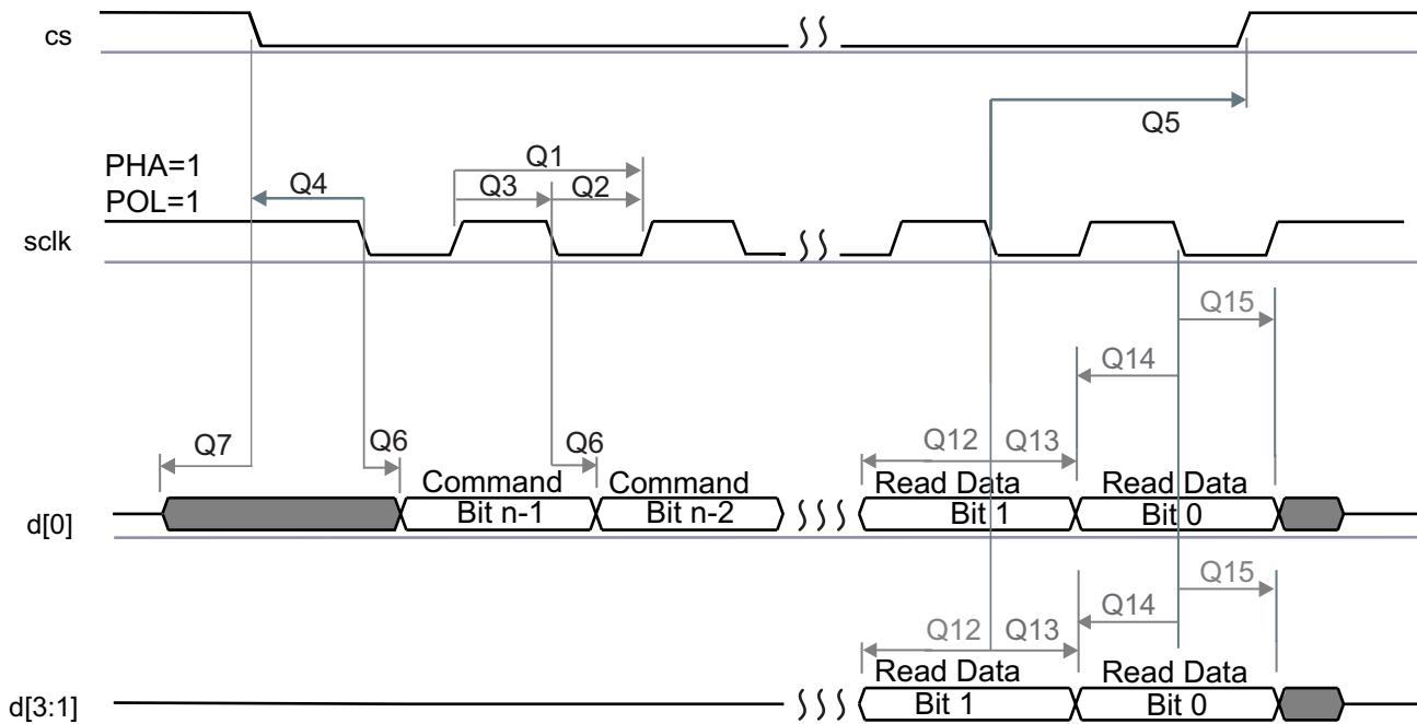
图 5-46. QSPI Read (Clock Mode 3)
