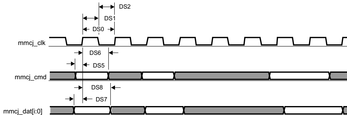
图 5-91. MMC/SD/SDIOj in - Default Speed - Receiver Mode
