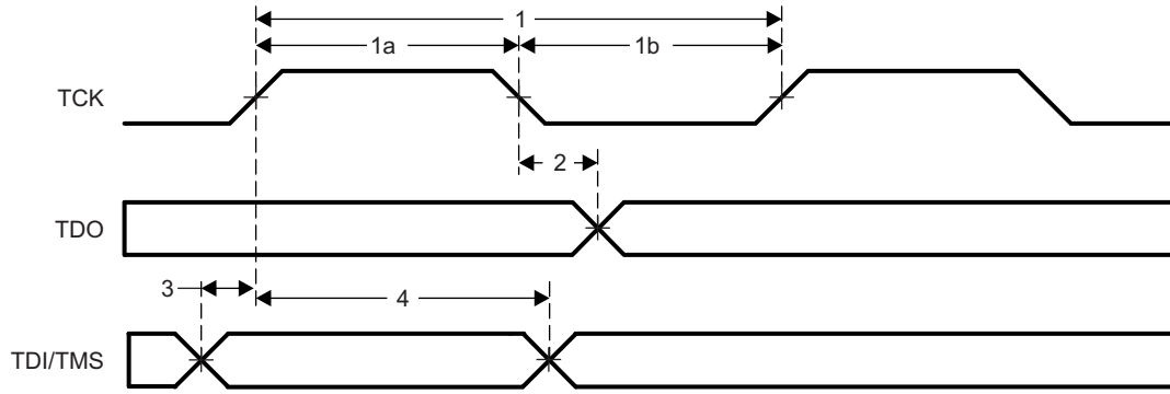
图 5-101. JTAG Timing
