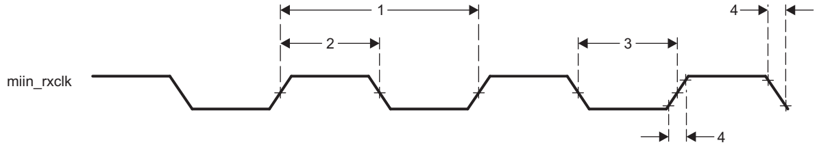
图 5-61. Clock Timing (GMAC Receive) - MII operation
