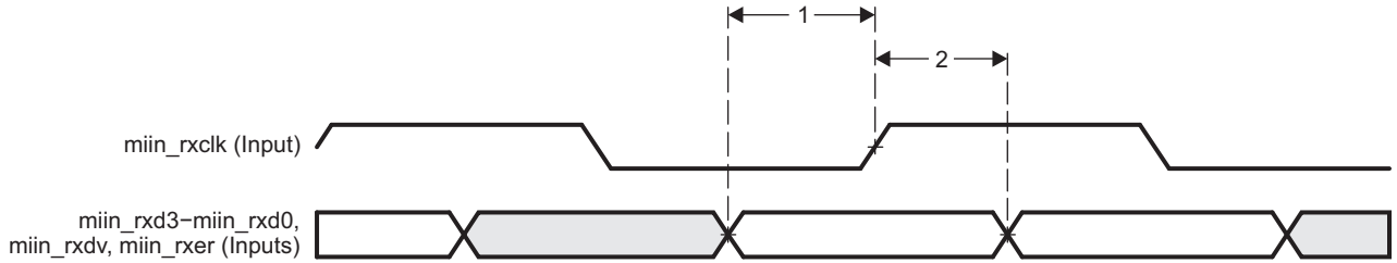
图 5-63. GMAC Receive Interface Timing MIIn operation
