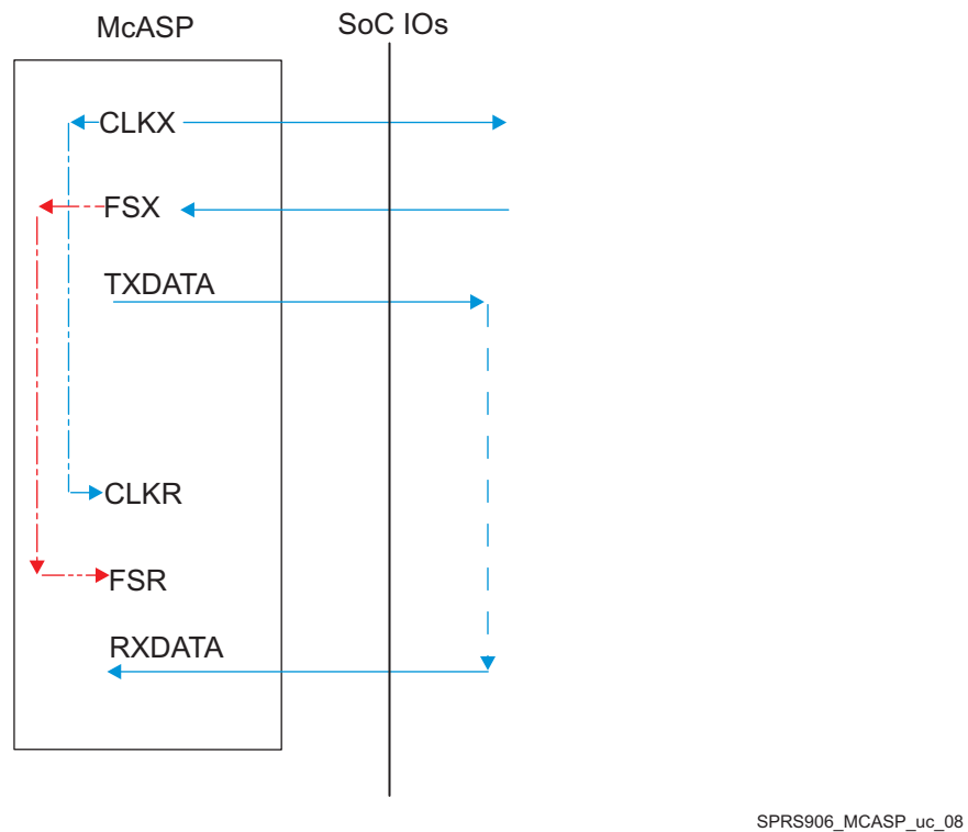
图 5-59. McASP1-8 CO-FI – SYNC Mode
