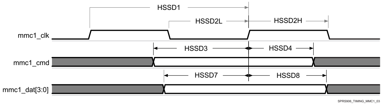
图 5-72. MMC/SD/SDIO in - High Speed - Receiver Mode
