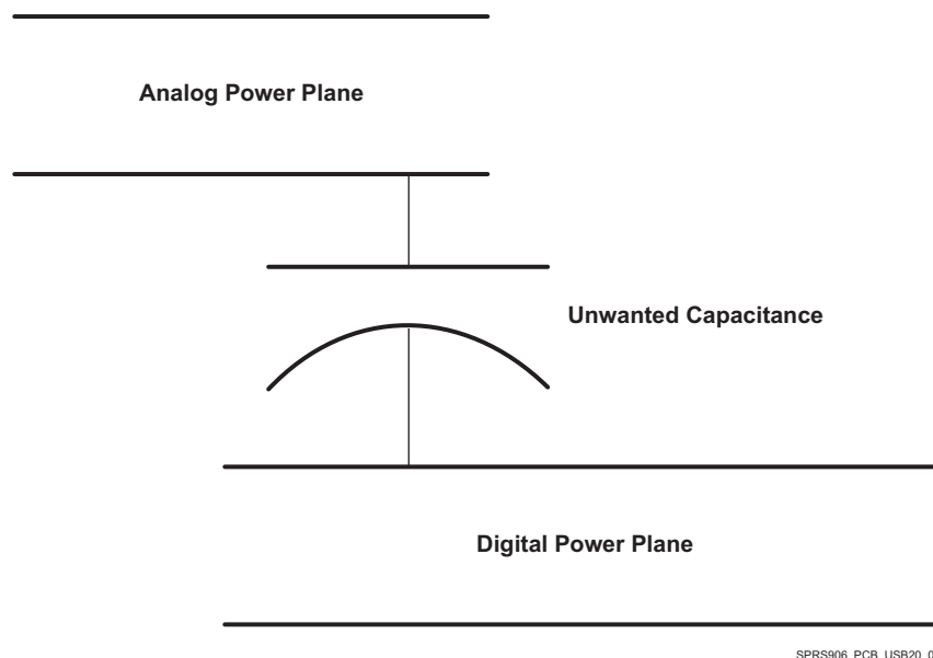
图 7-28. Do Not Overlap Planes
