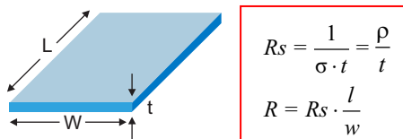
图 7-3. Depiction of Sheet Resistivity and Resistance
