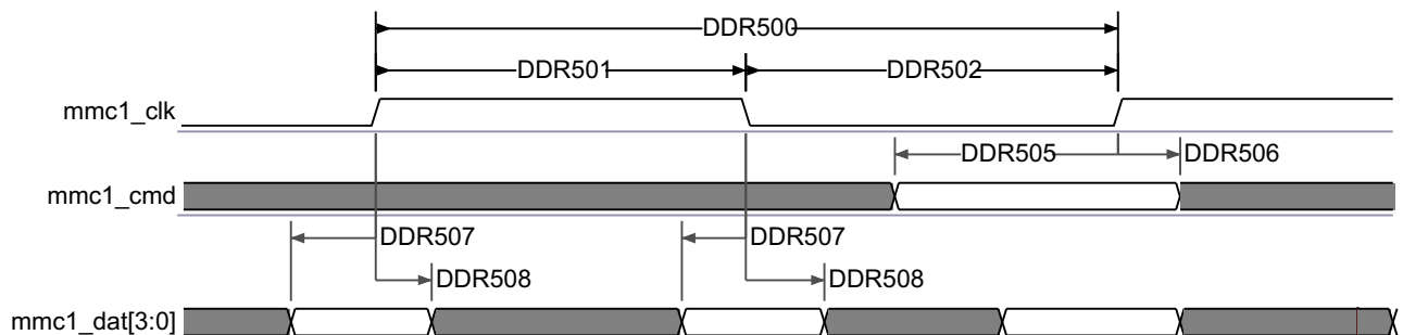
图 5-82. SDMMC - High Speed SD - DDR - Data/Command Receive
