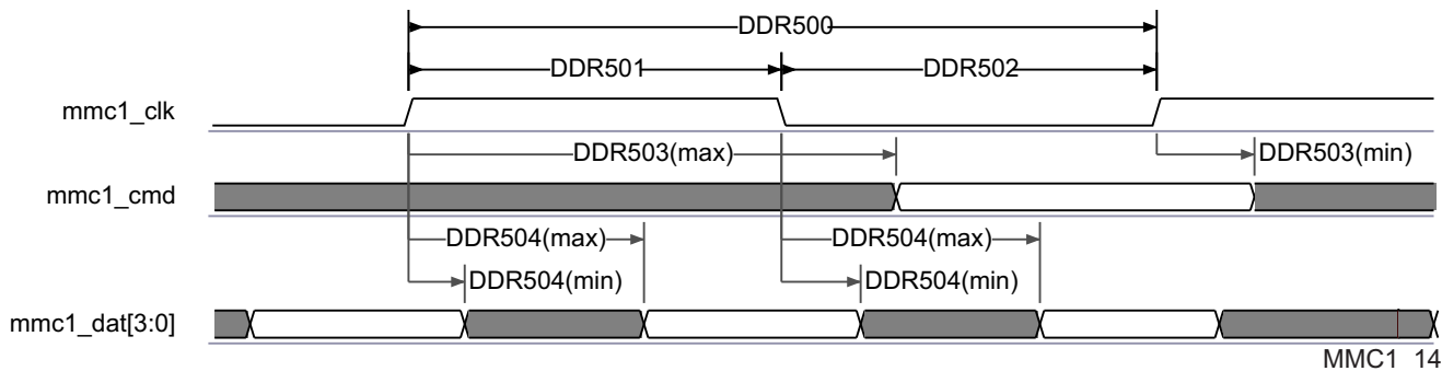
图 5-83. SDMMC - High Speed SD - DDR - Data/Command Transmit
