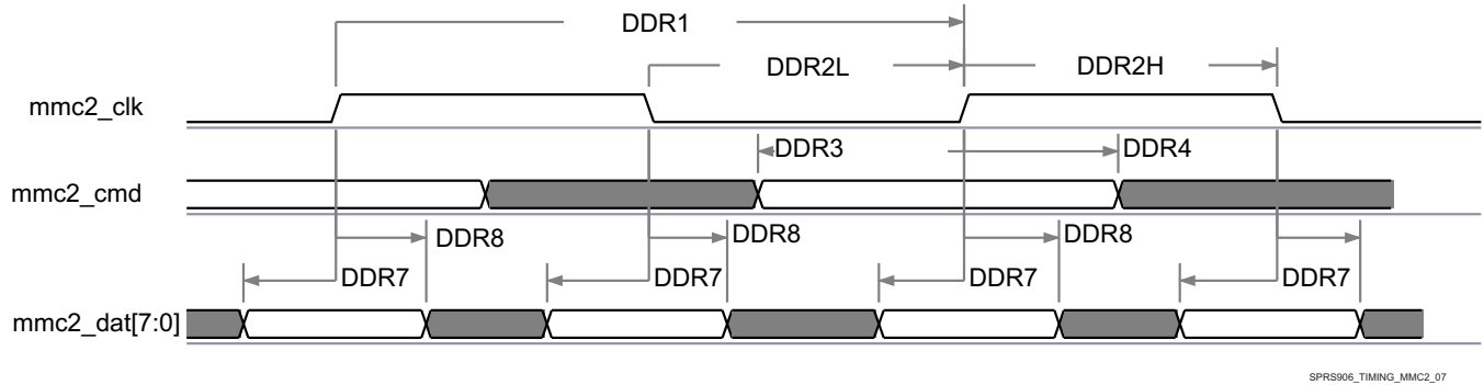
图 5-89. MMC/SD/SDIO in - High Speed DDR JC64 - Receiver Mode
