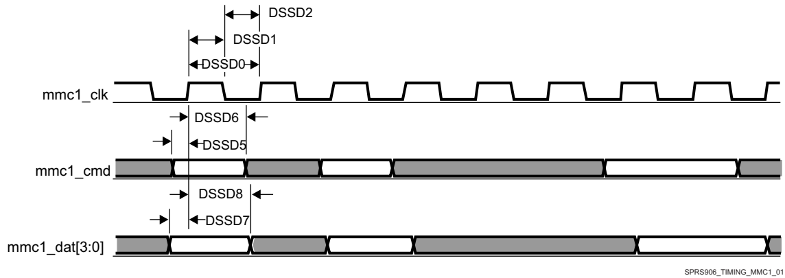
图 5-70. MMC/SD/SDIO in - Default Speed - Receiver Mode
