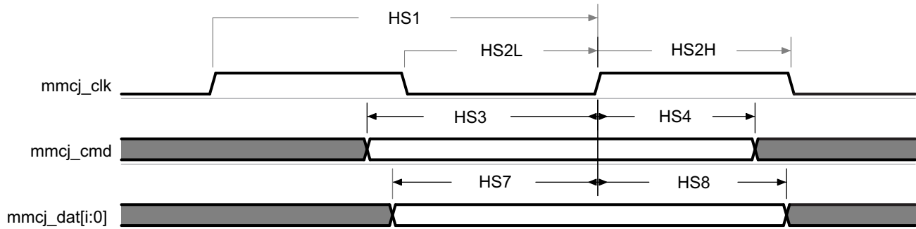
图 5-93. MMC/SD/SDIOj in - High Speed 3.3V Signaling - Receiver Mode
