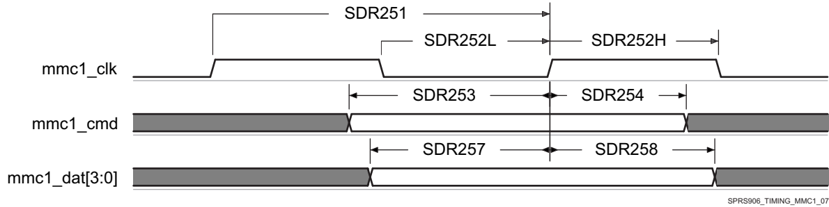
图 5-76. MMC/SD/SDIO in - High Speed SDR25 - Receiver Mode
