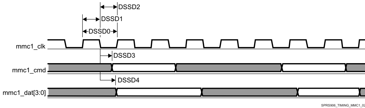
图 5-71. MMC/SD/SDIO in - Default Speed - Transmitter Mode
