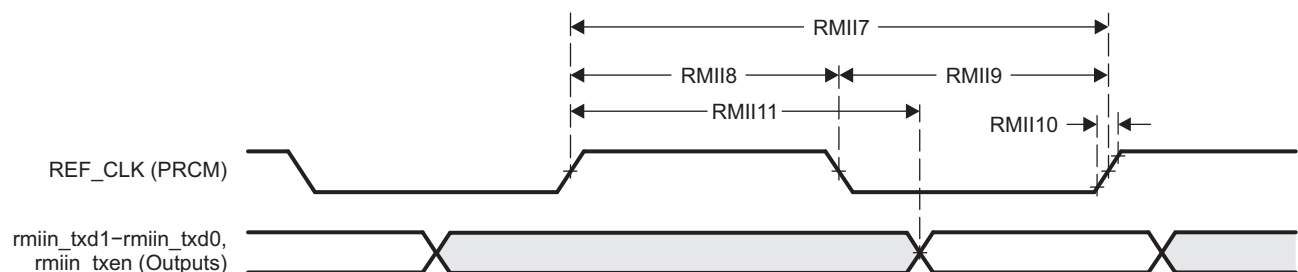
图 5-67. GMAC Transmit Interface Timing RMIIIn Operation
