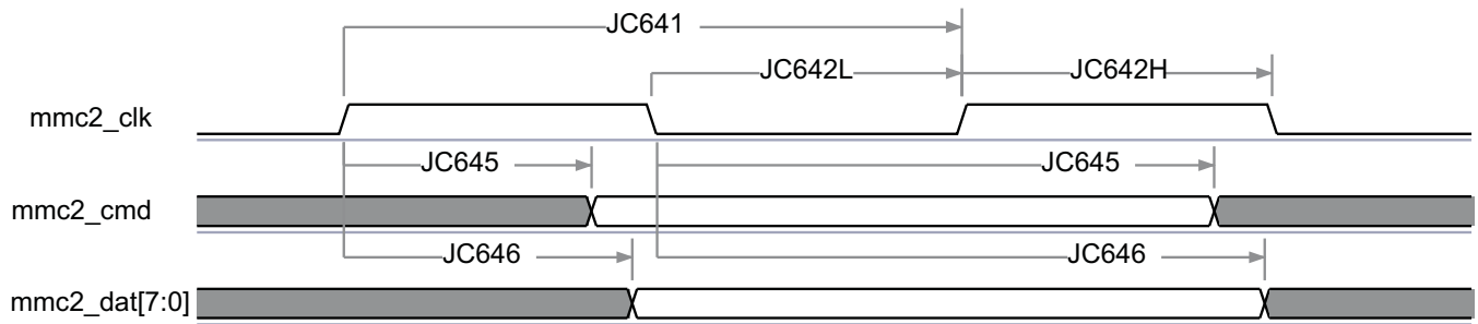
图 5-87. MMC/SD/SDIO in - High Speed JC64 - transmitter Mode
