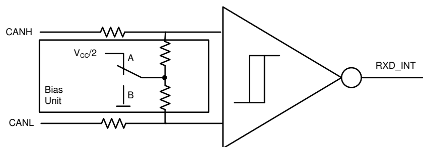
4. Simplified Recessive Common Mode Bias Unit and Receiver
