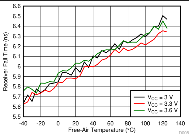
图 5-10. Receiver Fall Time vs Free-Air Temperature
