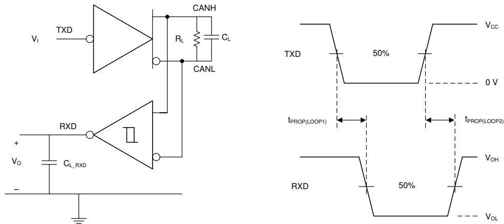
图 6-6. t_{\text{PROP(LOOP)}} Test Circuit and Measurement
