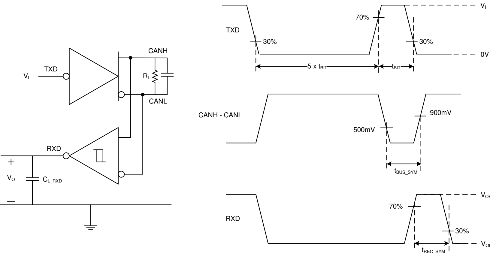
图 6-7. Loop Delay Symmetry Test Circuit and Measurement
