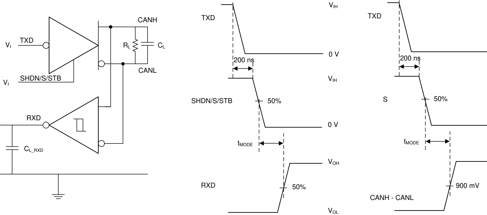
图 6-5. t_{\text{MODE}} Test Circuit and Measurement, from Shutdown, Standby or Silent to Normal Mode
