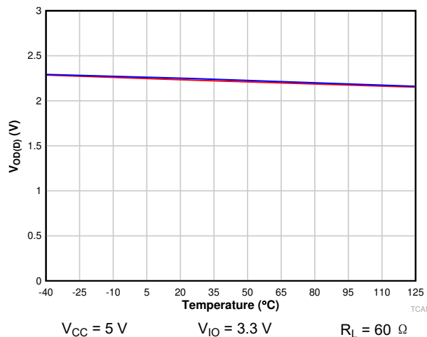
图 6-1. V_{OD(DOM)} Over Temperature V_{OD(DOM)} vs V_{CC} Transceiver 1 and Transceiver 2
