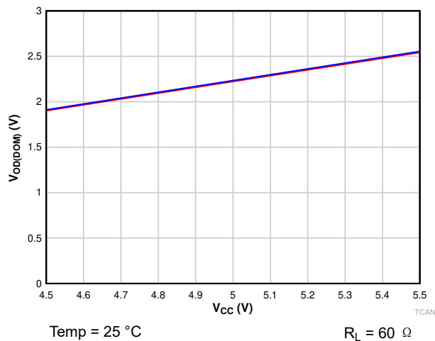
图 6-2. V_{OD(DOM)} Over V_{CC} V_{OD(DOM)} vs V_{CC} Transceiver 1 and Transceiver 2
