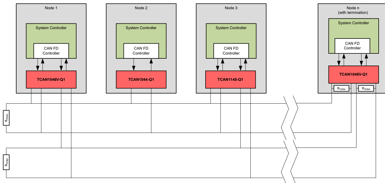
图 9-3. Typical CAN Bus
