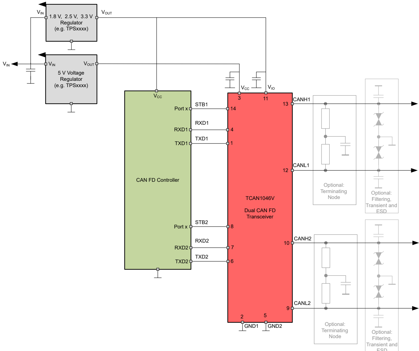
图 9-6. Transceiver Application Using 1.8 V, 2.5 V, 3.3 V I/O Connections
