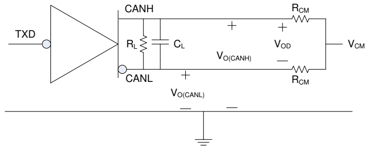
图 7-2. Driver Test Circuit and Measurement
