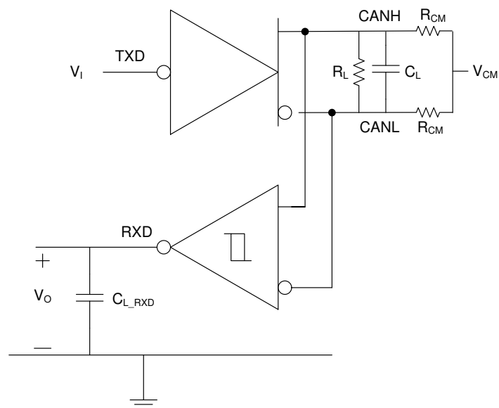
图 7-6. t_{PROP(LOOP)} Test Circuit and Measurement
