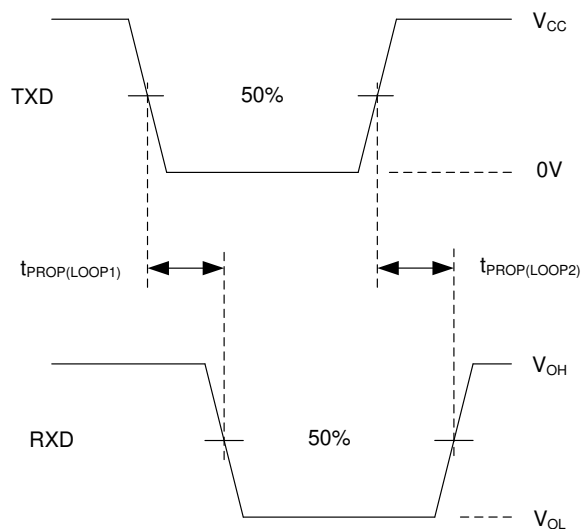
图 7-6. t_{PROP(LOOP)} Test Circuit and Measurement
