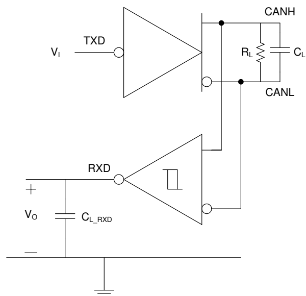
图 7-6. t_{PROP(LOOP)} Test Circuit and Measurement
