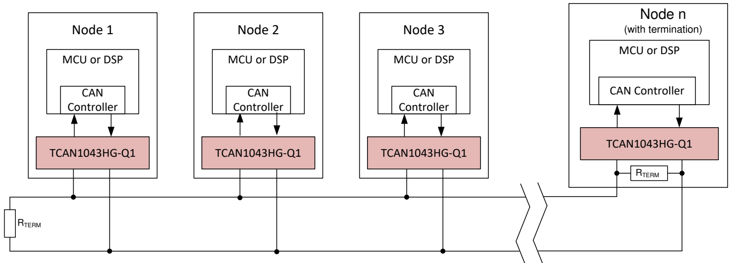
图 9-3. Typical CAN Bus Application
