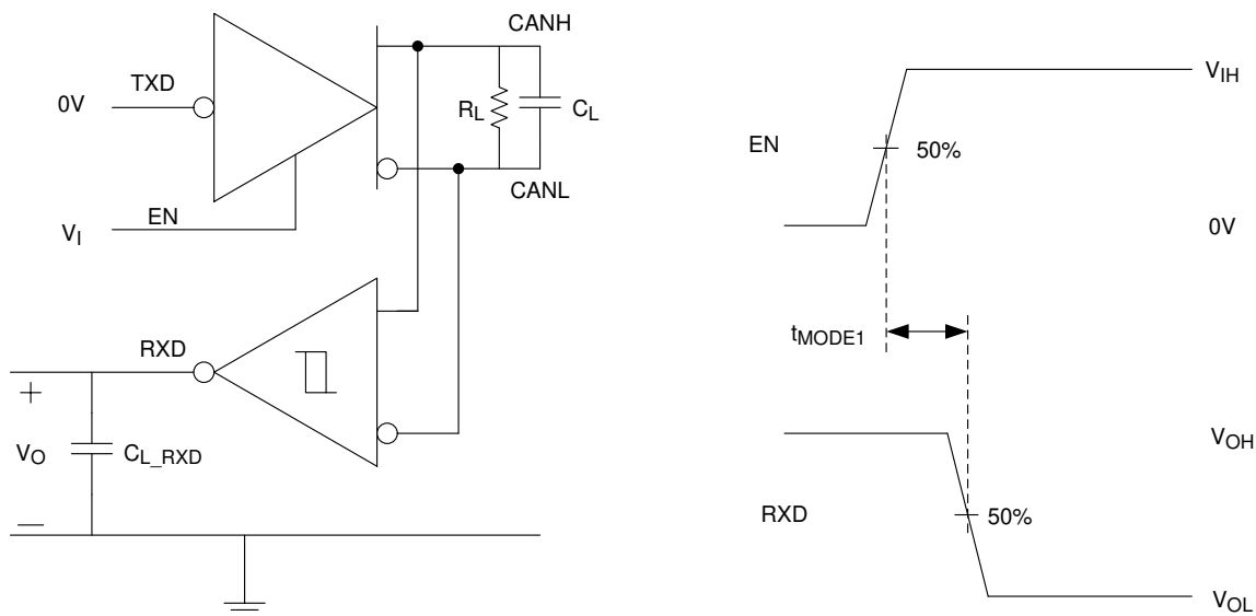
图 7-4. t_{\text{MODE1}} Test Circuit and Measurement, Silent Mode to Normal Mode
