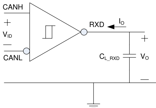
图 7-3. Receiver Test Circuit and Measurement
