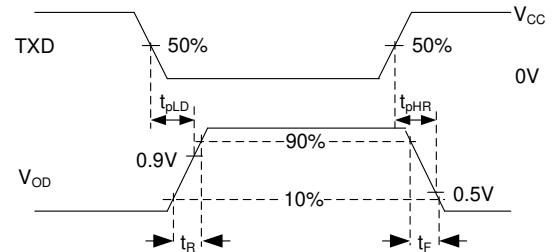
图 7-2. Driver Test Circuit and Measurement
