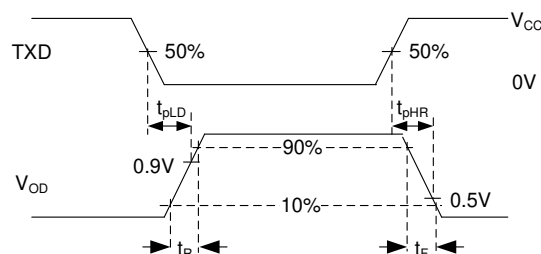
图 7-2. Driver Test Circuit and Measurement
