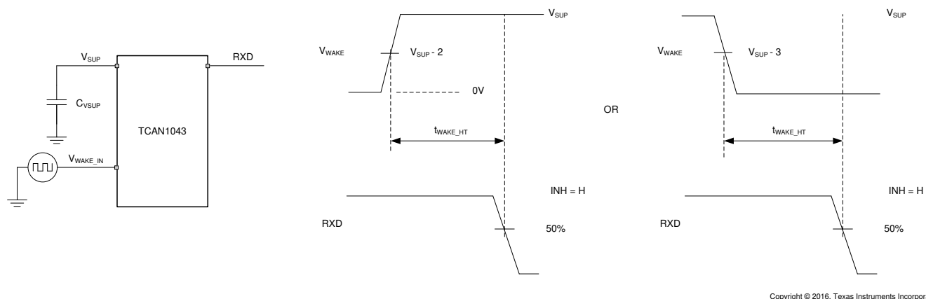
图 7-13. t_{WAKE\_HT} While Monitoring RXD Output
