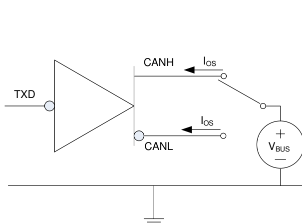
图 7-9. TXD Dominant Timeout Test Circuit and Measurement
