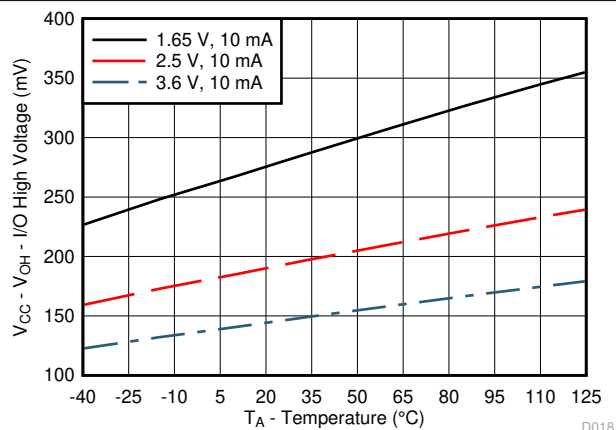
图 6-13. V_{CC} - V_{OH} Voltage vs Temperature for Different V_{CC} D018
