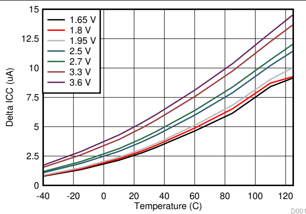
图 6-14. \Delta I_{CC} vs Temperature for Different V_{CC} ( V_I = V_{CC} - 0.6 V) D001
