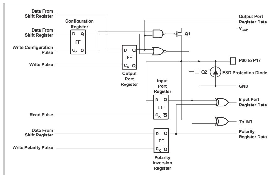
图 8-1. Logic Diagram (Positive Logic)
