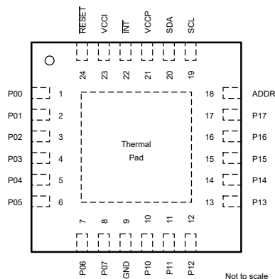
图 5-2. RTW Package, 24-Pin WQFN (Top View)
