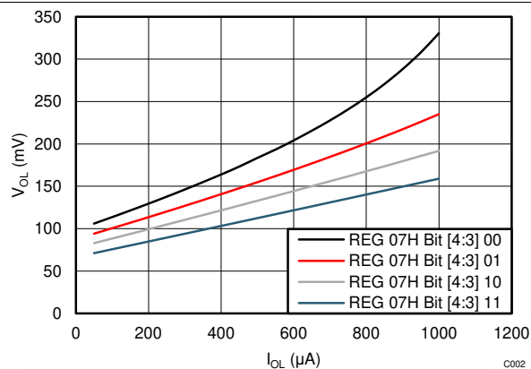
Figure 27. V_{OL} vs I_{OL} for User Card
