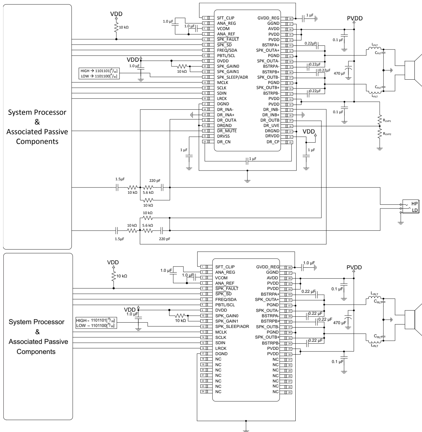
Figure 62. Mono PBTL Using Software Control
