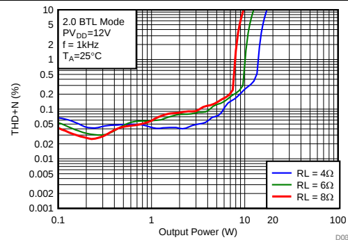
图 19. Total Harmonic Distortion + Noise vs Output Power
