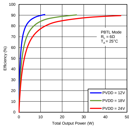
图 40. Efficiency vs Output Power (PBTL Mode)
