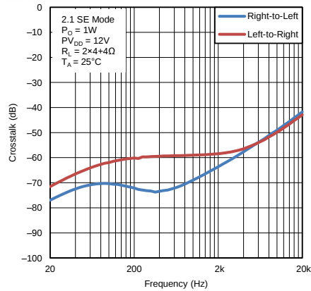
图 15. Crosstalk vs Frequency
