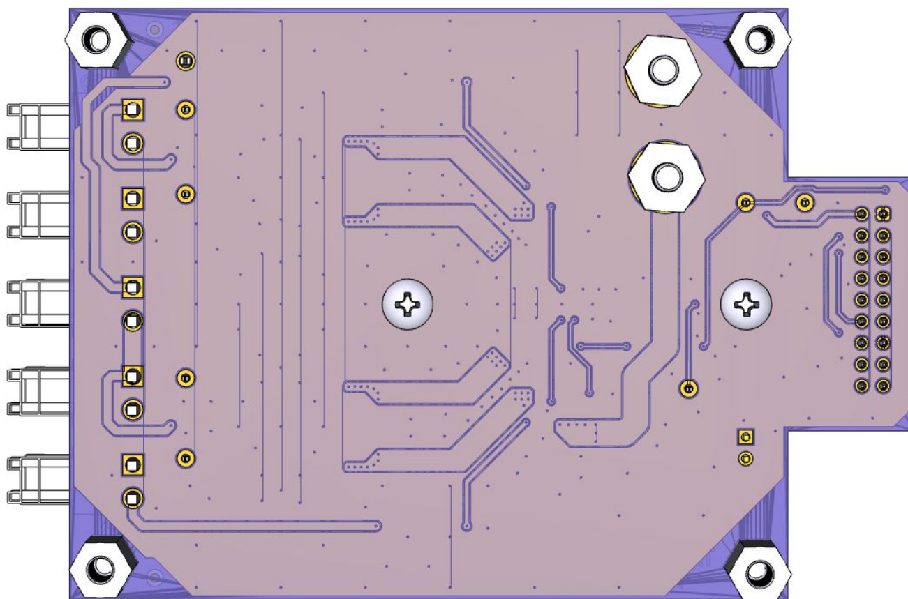
图 74. Bottom Layer Layout with Stereo BTL Mode
