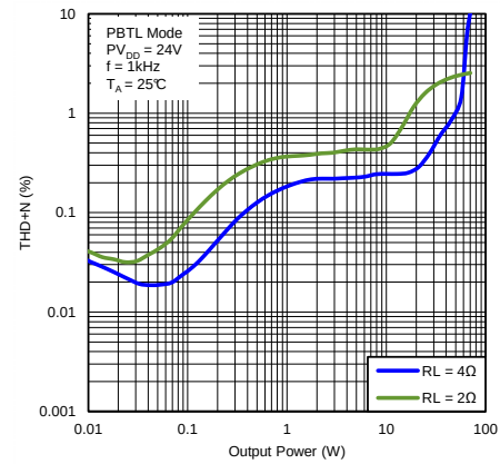
图 36. Total Harmonic Distortion + Noise vs Output Power (PBTL Mode)
