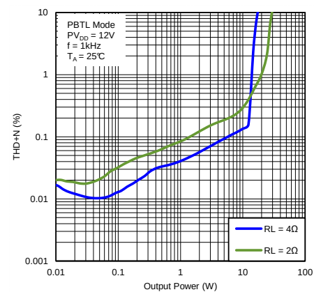
图 34. Total Harmonic Distortion + Noise vs Output Power (PBTL Mode)
