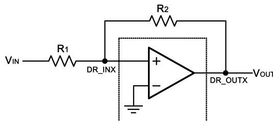
图 49. Headphone/Line Amplifier
