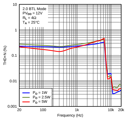
图 9. THD+N vs Frequency
