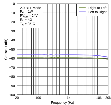
图 32. Crosstalk vs Frequency
