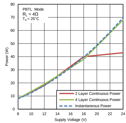
图 42. Power vs Supply Voltage (PBTL Mode)
