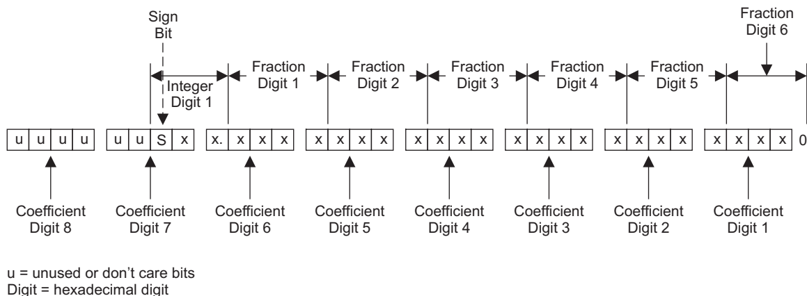
图 66. Alignment of 3.23 Coefficient in 32-Bit I 2 C Word
