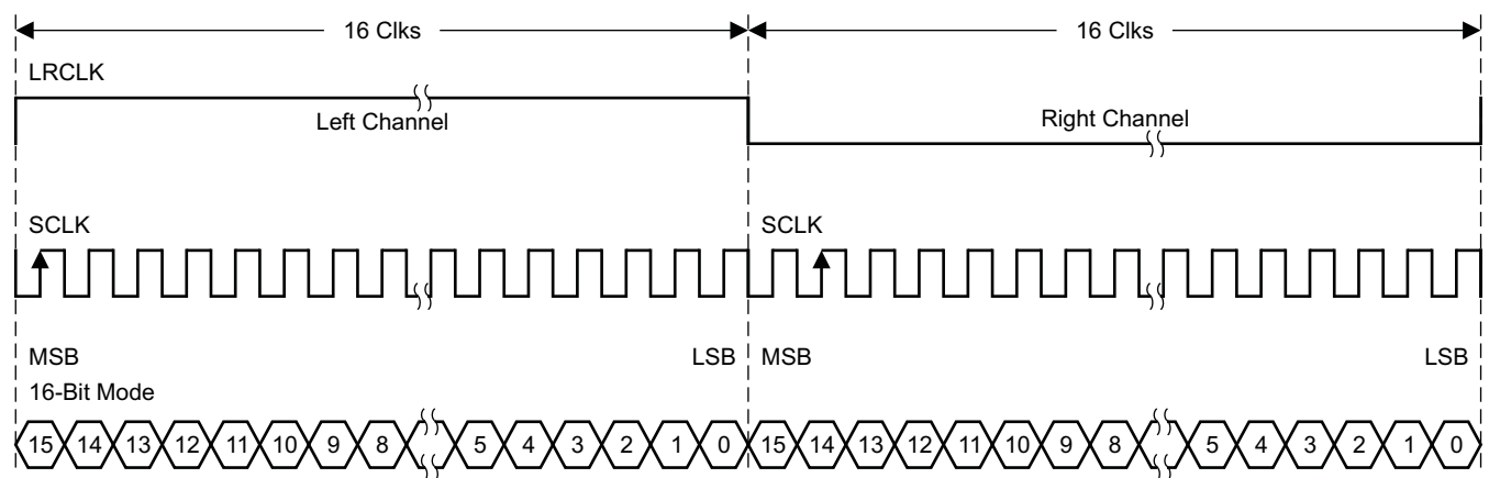
图 60. Left-Justified 32-f s Format
