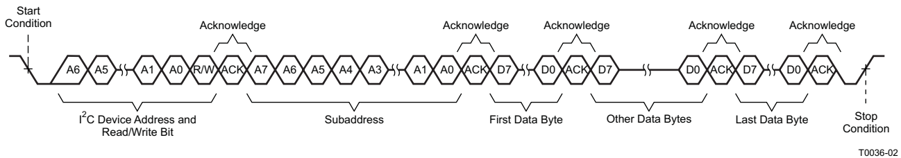
图 52. Multiple-Byte Write Transfer
