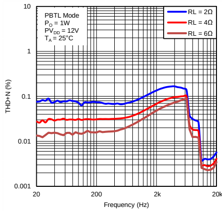
图 37. Total Harmonic Distortion + Noise vs Frequency (PBTL Mode)
