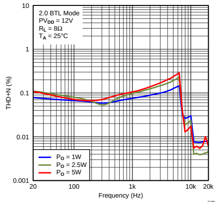
图 7. THD+N vs Frequency
