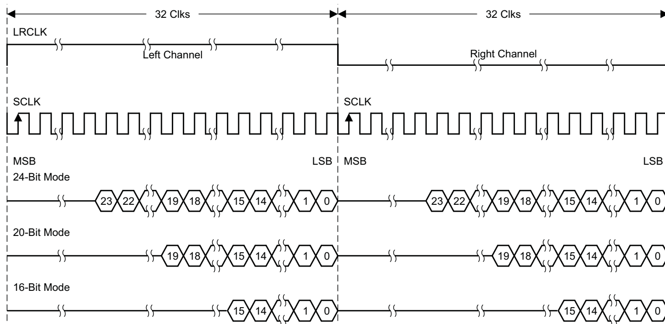
图 61. Right-Justified 64- f_s Format
