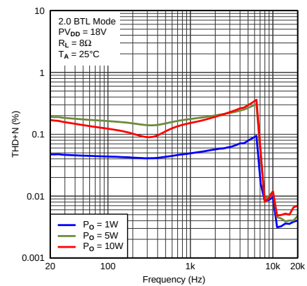
图 10. THD+N vs Frequency
