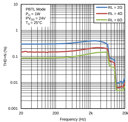
图 39. Total Harmonic Distortion + Noise vs Frequency (PBTL Mode)
