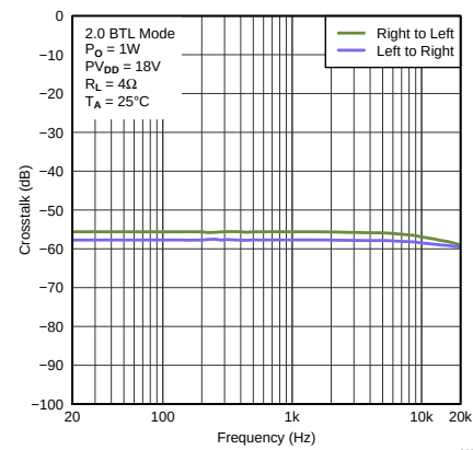
图 30. Crosstalk vs Frequency
