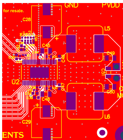
图 73. Layout Example (Mono) - Top View Composite
