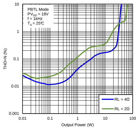
图 35. Total Harmonic Distortion + Noise vs Output Power (PBTL Mode)
