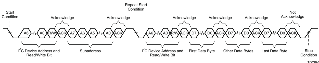
图 54. Multiple-Byte Read Transfer
