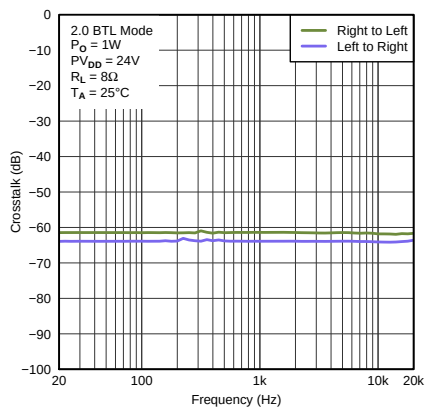
图 31. Crosstalk vs Frequency
