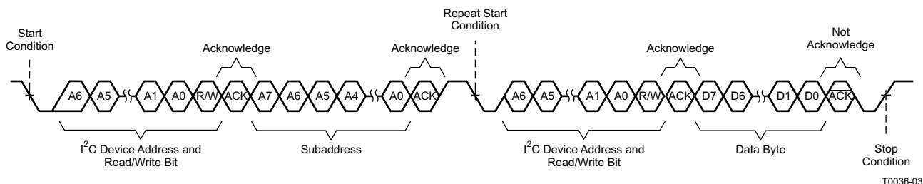
图 53. Single-Byte Read Transfer
