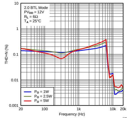
图 8. THD+N vs Frequency
