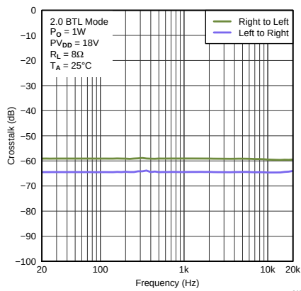
图 29. Crosstalk vs Frequency
