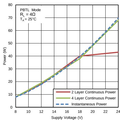
图 33. Output Power vs Supply Voltage (PBTL Mode)
