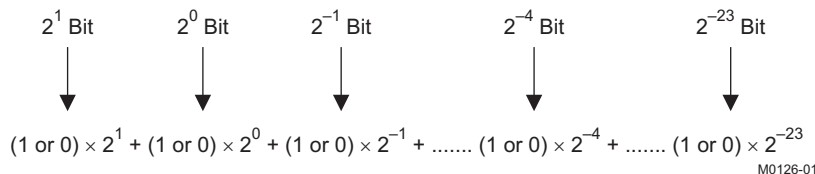
图 65. Conversion Weighting Factors—3.23 Format to Floating Point
