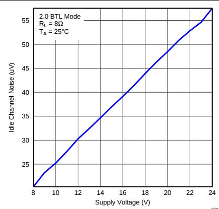
图 6. Idle Channel Noise vs Supply Voltage
