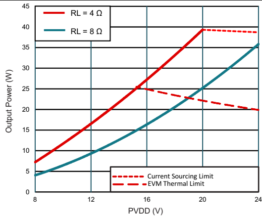
图 5. Output Power vs Supply Voltage
