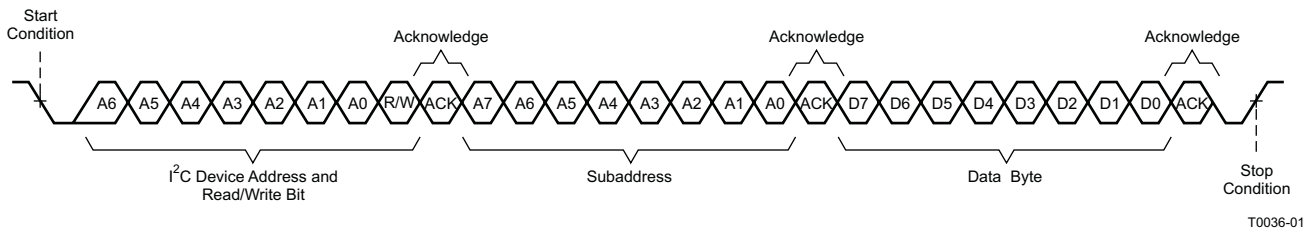
图 51. Single-Byte Write Transfer
