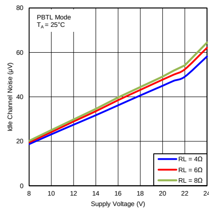
图 43. Idle Channel Noise vs Supply Voltage (PBTL Mode)
