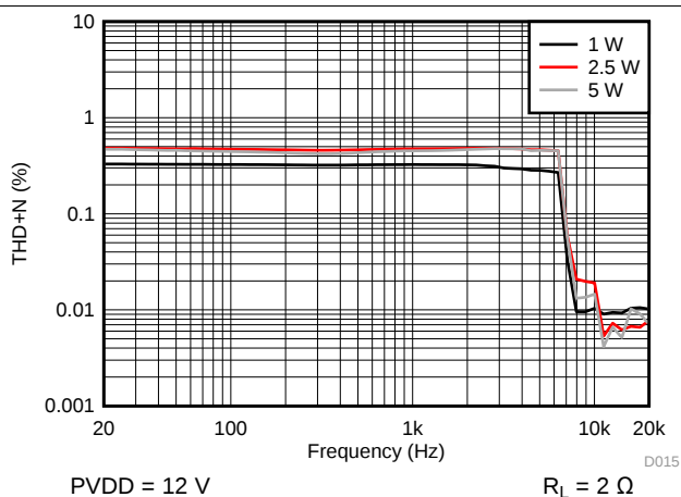
图 19. THD+N vs Frequency - PBTl
