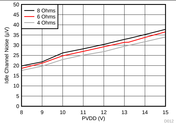
图 6. Idle Channel Noise vs Supply Voltage - BTL
