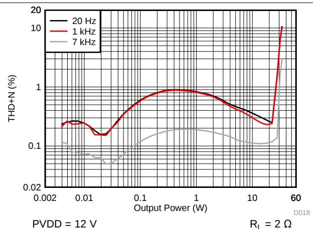
图 22. THD+N vs Output Power - PBTl
