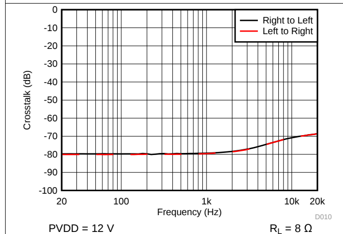
图 15. Crosstalk vs Frequency - BTL
