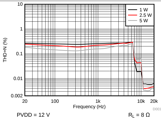
图 7. THD+N vs Frequency - BTL
