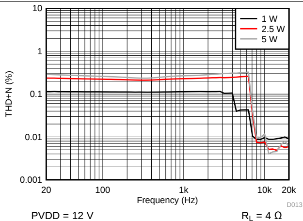
图 17. THD+N vs Frequency - PBTl
