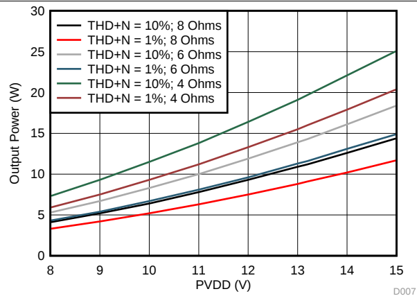
图 5. Output Power vs Supply Voltage - BTL
