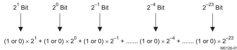
图 47. Conversion Weighting Factors—3.23 Format to Floating Point
