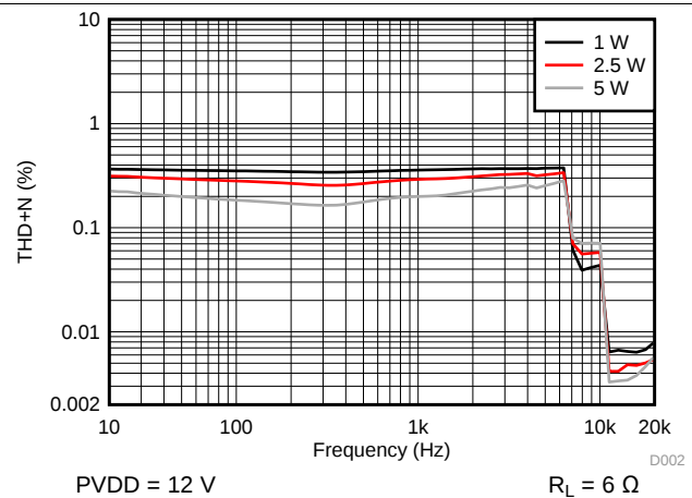
图 8. THD+N vs Frequency - BTL
