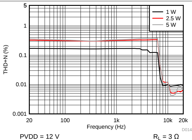
图 18. THD+N vs Frequency - PBTl
