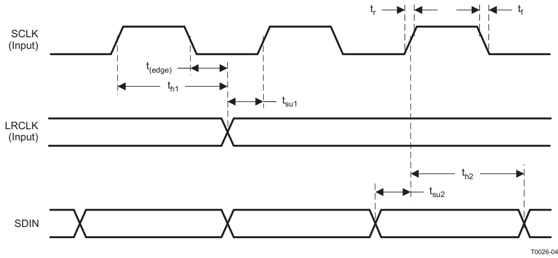
图 4. Serial Audio Port Timing
