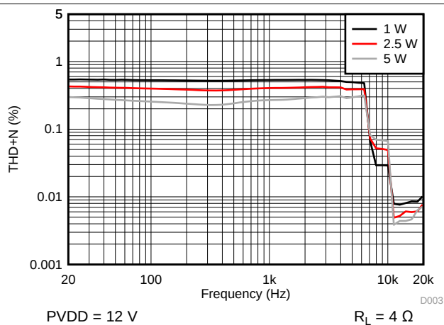
图 9. THD+N vs Frequency - BTL
