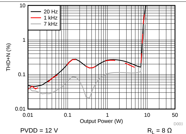
图 10. THD+N vs Output Power - BTL
