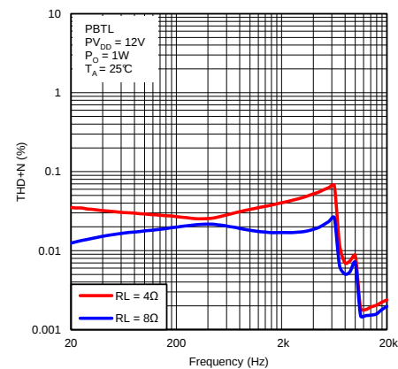
Figure 8. Total Harmonic Distortion + Noise vs Frequency in Post-Filter PBTL Mode With PVDD = 12 V
