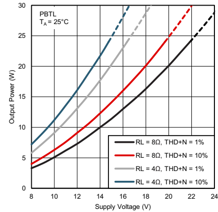
Figure 4. Output Power vs PVDD in Post-Filter PBTL Mode
