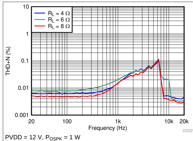
Figure 1. THD+N vs Frequency
